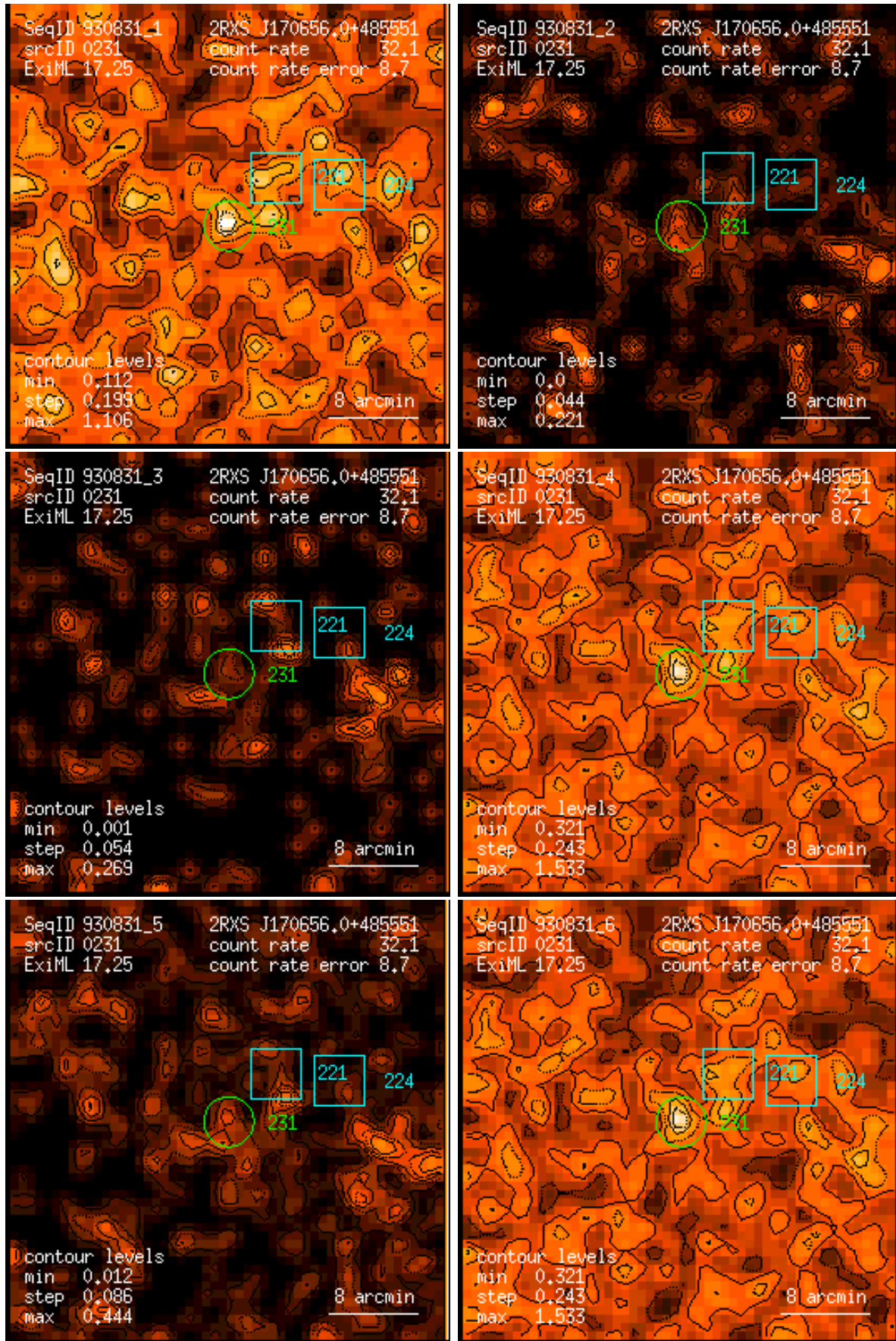
Figure 231: RASS 930831: detection 0231: band rate images, Gaussian filter: (1) PSPC channels 11 – 41, (2) 52 – 90, (3) 91 – 201, (4) 11 – 235, (5) 52 – 201, (6) 11 – 201. Broad band rates in counts/ks. Band rate contour levels in counts/ks/arcmin 2 .
