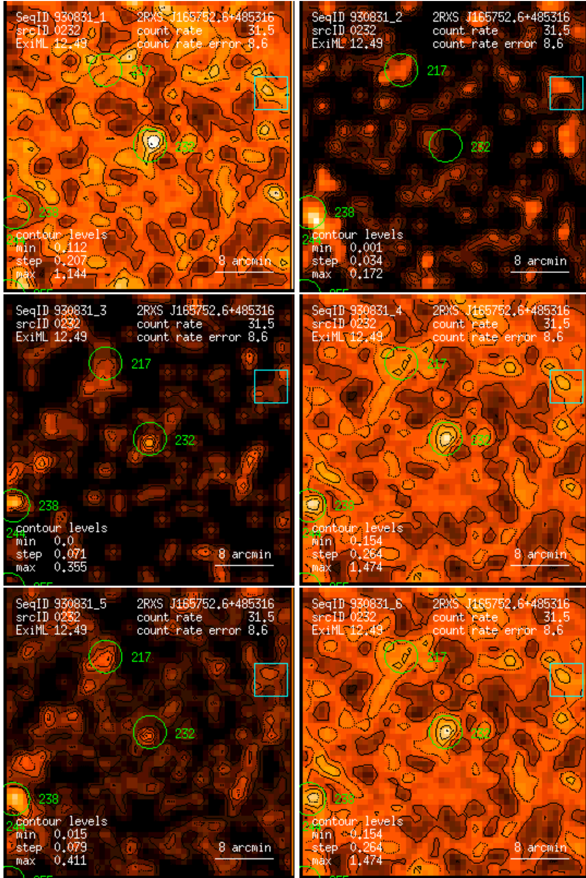
Figure 232: RASS 930831: detection 0232: band rate images, Gaussian filter: (1) PSPC channels 11 – 41, (2) 52 – 90, (3) 91 – 201, (4) 11 – 235, (5) 52 – 201, (6) 11 – 201. Broad band rates in counts/ks. Band rate contour levels in counts/ks/arcmin 2 .
