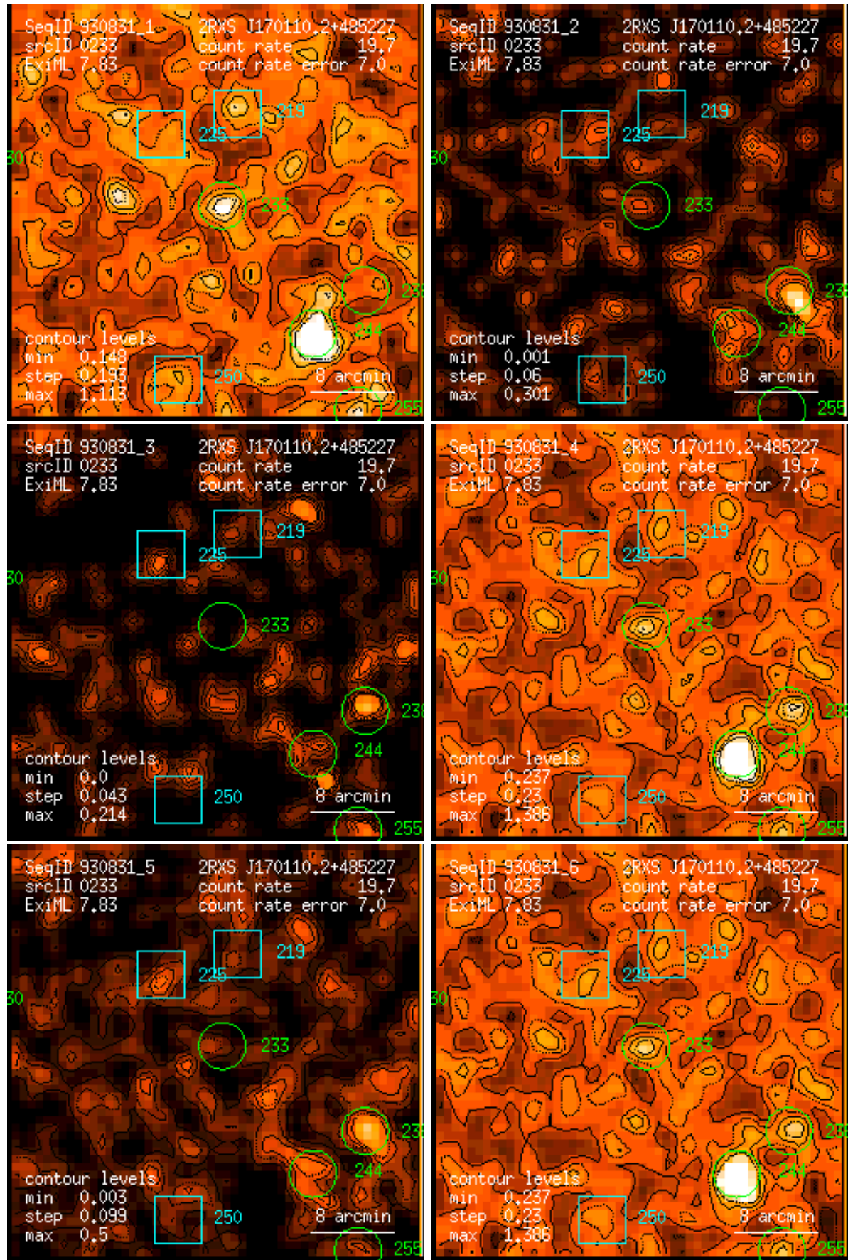
Figure 233: RASS 930831: detection 0233: band rate images, Gaussian filter: (1) PSPC channels 11 – 41, (2) 52 – 90, (3) 91 – 201, (4) 11 – 235, (5) 52 – 201, (6) 11 – 201. Broad band rates in counts/ks. Band rate contour levels in counts/ks/arcmin 2 .
