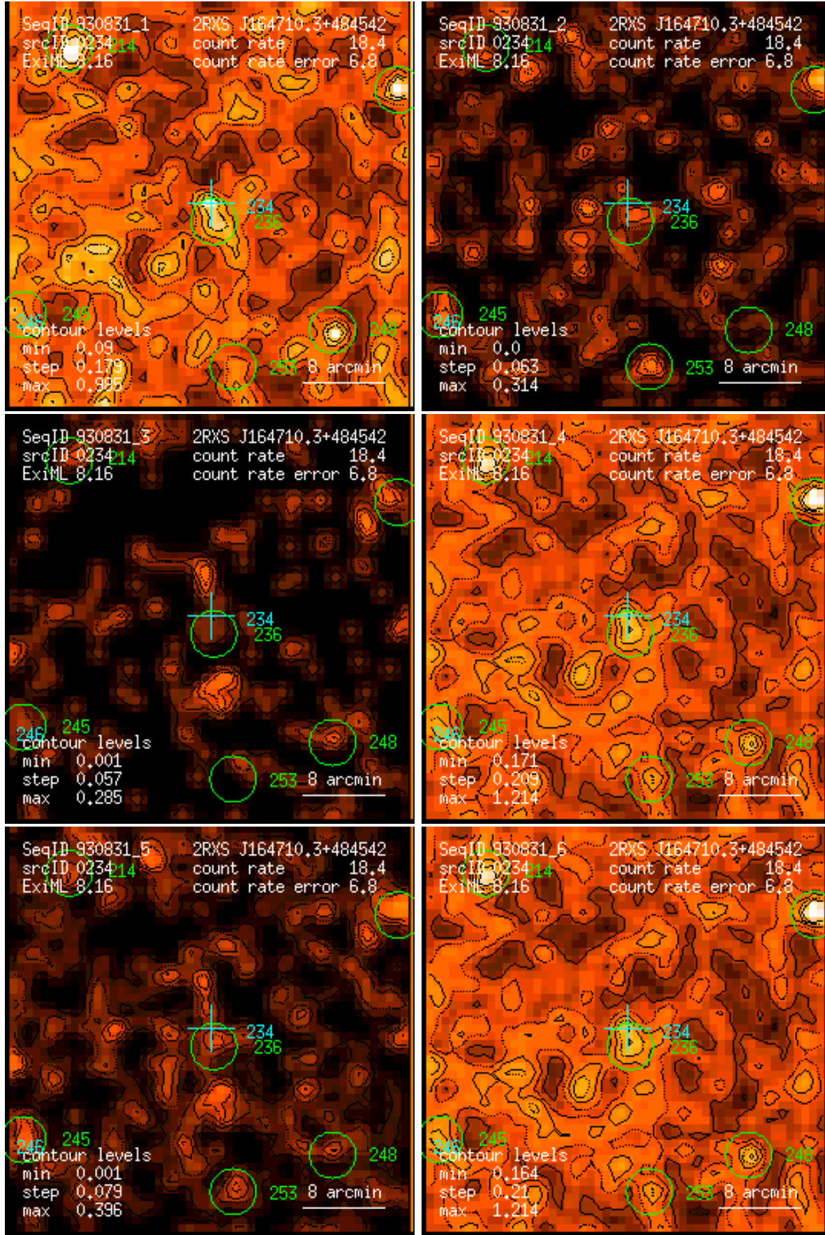
Figure 234: RASS 930831: detection 0234: band rate images, Gaussian filter: (1) PSPC channels 11 – 41, (2) 52 – 90, (3) 91 – 201, (4) 11 – 235, (5) 52 – 201, (6) 11 – 201. Broad band rates in counts/ks. Band rate contour levels in counts/ks/arcmin 2 .
