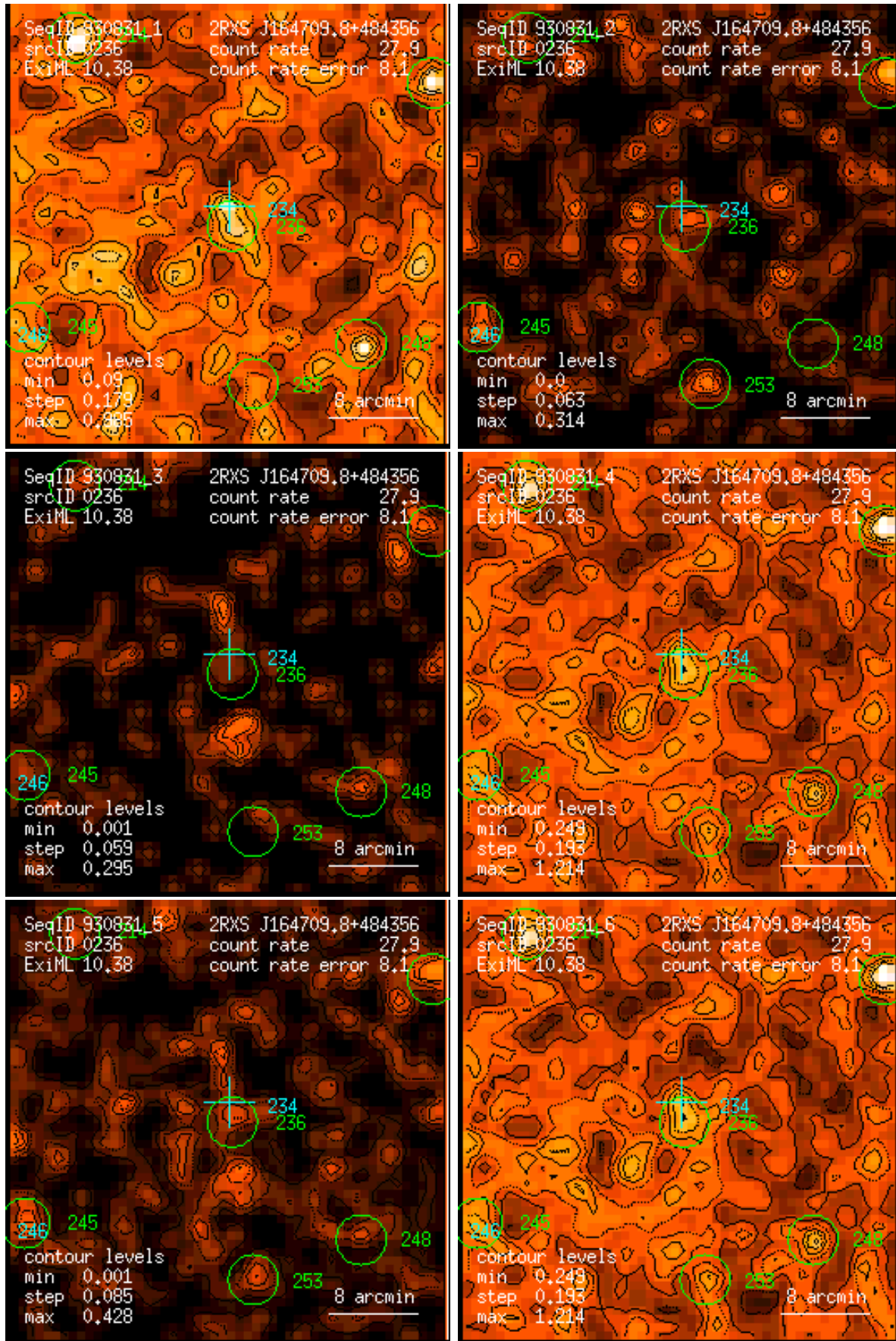
Figure 236: RASS 930831: detection 0236: band rate images, Gaussian filter: (1) PSPC channels 11 – 41, (2) 52 – 90, (3) 91 – 201, (4) 11 – 235, (5) 52 – 201, (6) 11 – 201. Broad band rates in counts/ks. Band rate contour levels in counts/ks/arcmin 2 .
