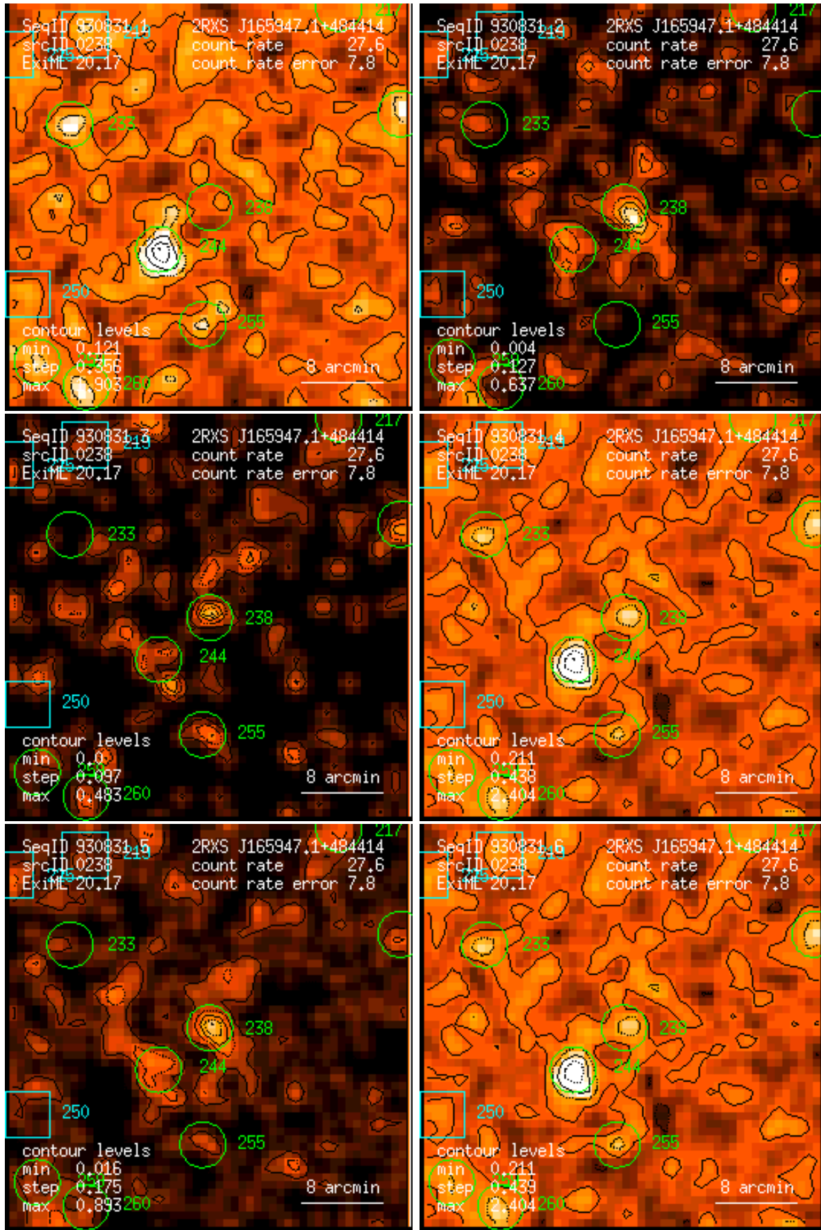
Figure 238: RASS 930831: detection 0238: band rate images, Gaussian filter: (1) PSPC channels 11 – 41, (2) 52 – 90, (3) 91 – 201, (4) 11 – 235, (5) 52 – 201, (6) 11 – 201. Broad band rates in counts/ks. Band rate contour levels in counts/ks/arcmin 2 .
