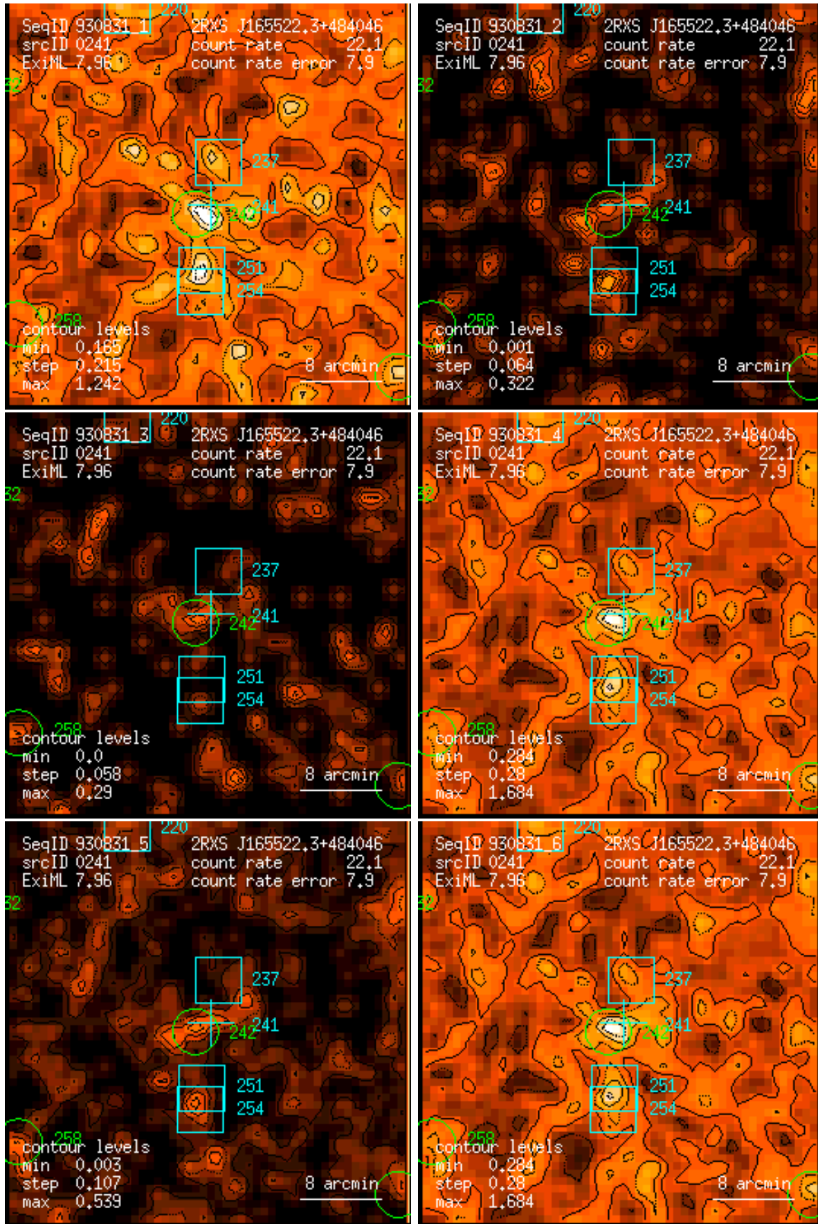
Figure 241: RASS 930831: detection 0241: band rate images, Gaussian filter: (1) PSPC channels 11 – 41, (2) 52 – 90, (3) 91 – 201, (4) 11 – 235, (5) 52 – 201, (6) 11 – 201. Broad band rates in counts/ks. Band rate contour levels in counts/ks/arcmin 2 .
