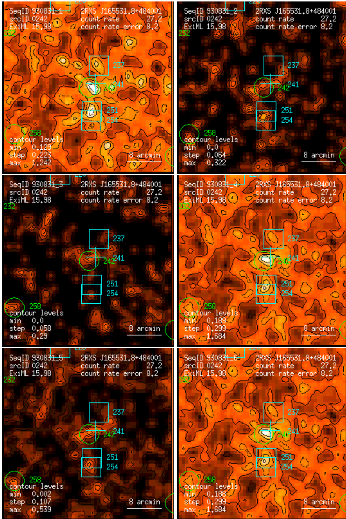
Figure 242: RASS 930831: detection 0242: band rate images, Gaussian filter: (1) PSPC channels 11 – 41, (2) 52 – 90, (3) 91 – 201, (4) 11 – 235, (5) 52 – 201, (6) 11 – 201. Broad band rates in counts/ks. Band rate contour levels in counts/ks/arcmin 2 .
