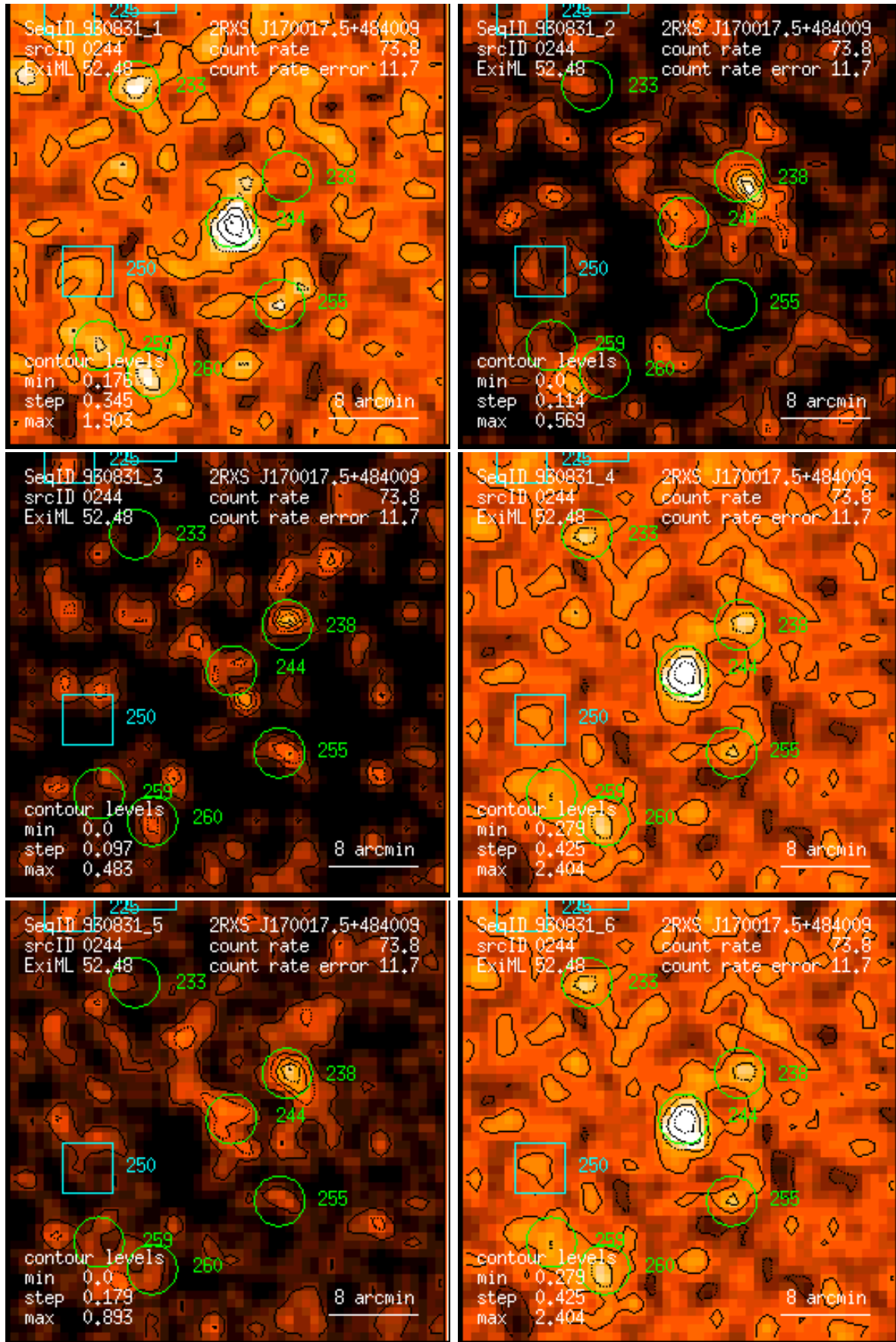
Figure 244: RASS 930831: detection 0244: band rate images, Gaussian filter: (1) PSPC channels 11 – 41, (2) 52 – 90, (3) 91 – 201, (4) 11 – 235, (5) 52 – 201, (6) 11 – 201. Broad band rates in counts/ks. Band rate contour levels in counts/ks/arcmin 2 .
