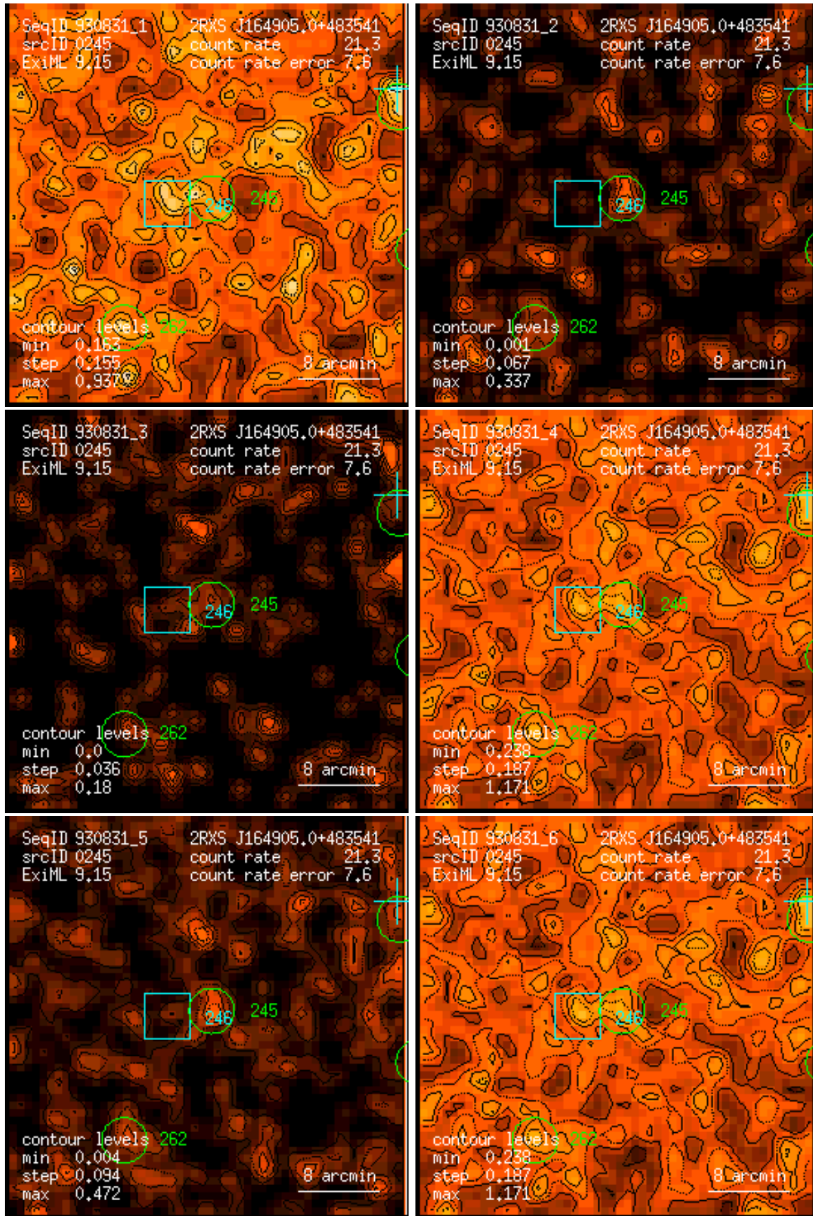
Figure 245: RASS 930831: detection 0245: band rate images, Gaussian filter: (1) PSPC channels 11 – 41, (2) 52 – 90, (3) 91 – 201, (4) 11 – 235, (5) 52 – 201, (6) 11 – 201. Broad band rates in counts/ks. Band rate contour levels in counts/ks/arcmin 2 .
