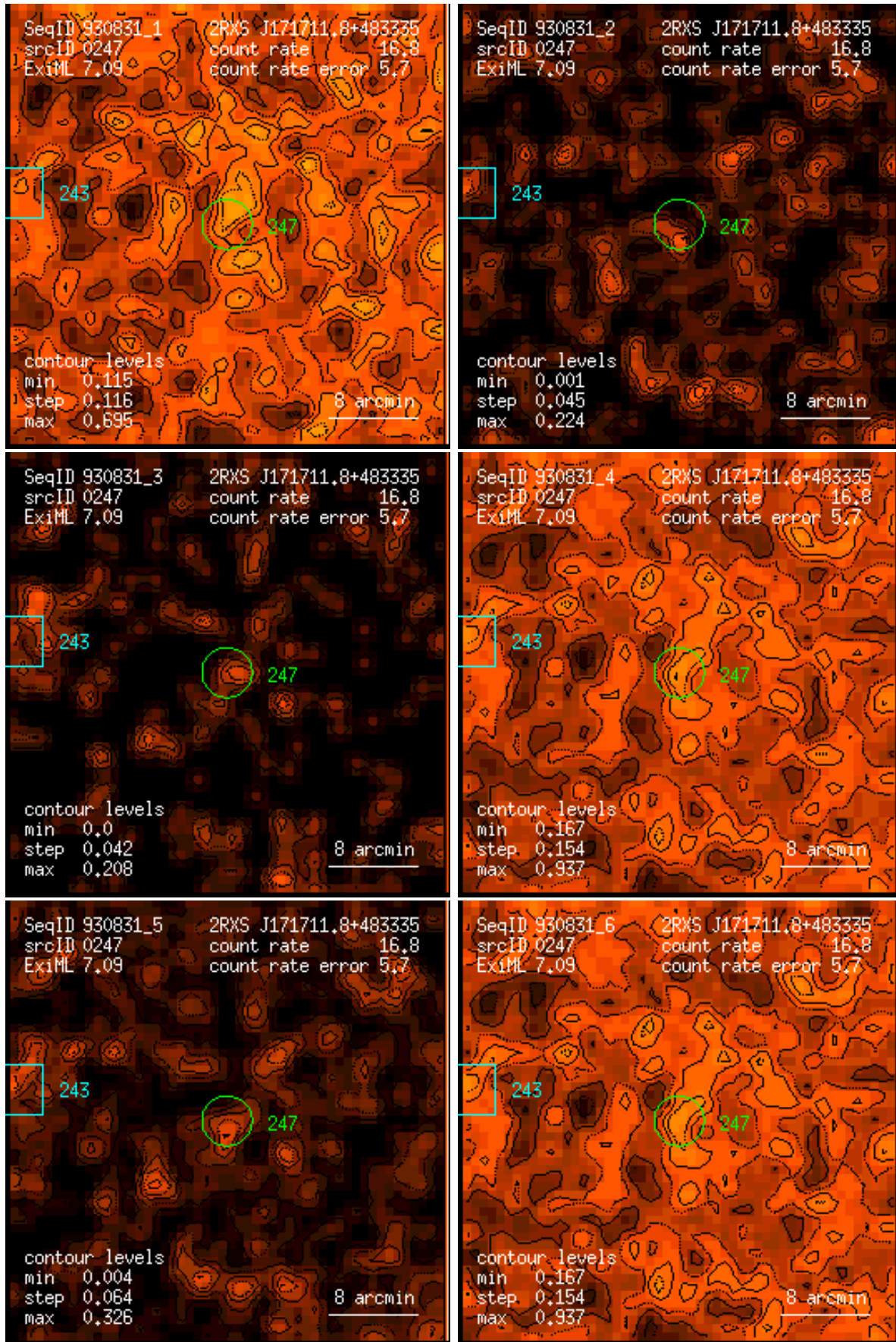
Figure 247: RASS 930831: detection 0247: band rate images, Gaussian filter: (1) PSPC channels 11 – 41, (2) 52 – 90, (3) 91 – 201, (4) 11 – 235, (5) 52 – 201, (6) 11 – 201. Broad band rates in counts/ks. Band rate contour levels in counts/ks/arcmin 2 .
