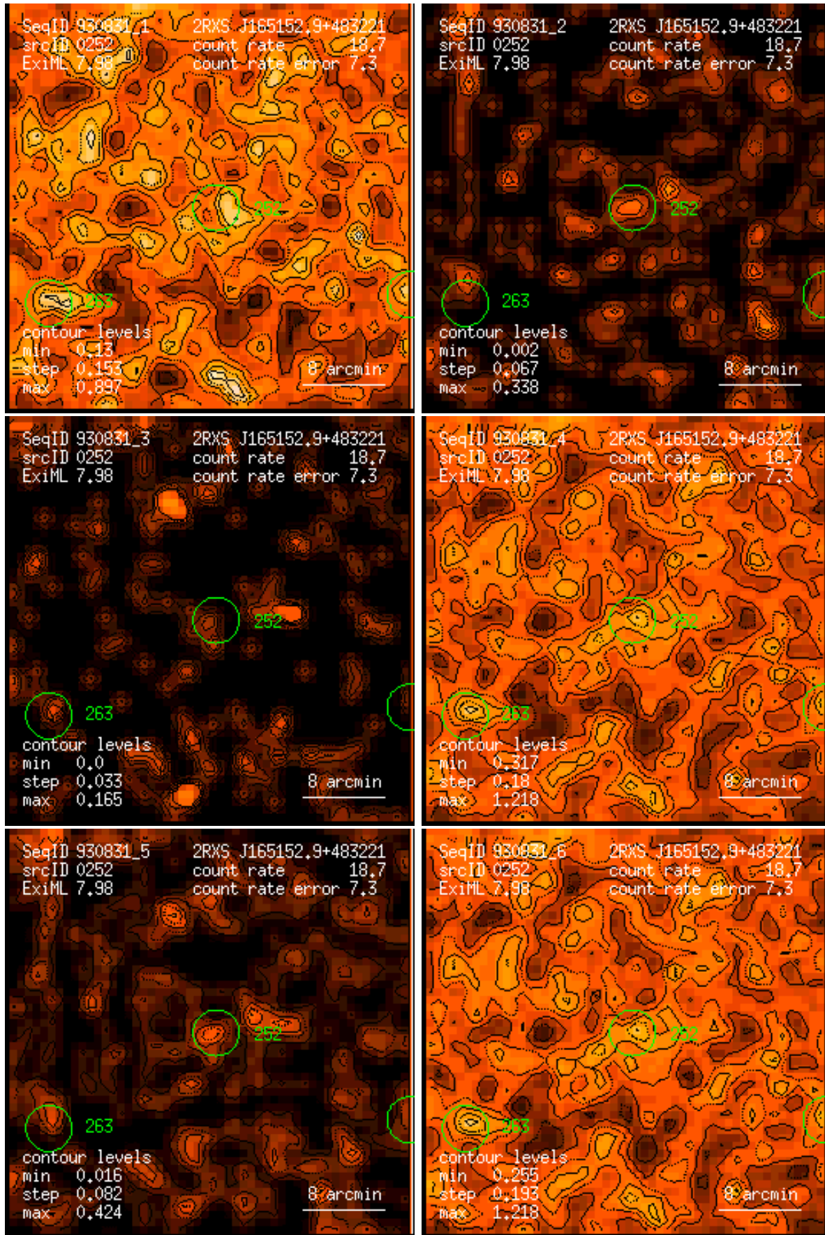
Figure 252: RASS 930831: detection 0252: band rate images, Gaussian filter: (1) PSPC channels 11 – 41, (2) 52 – 90, (3) 91 – 201, (4) 11 – 235, (5) 52 – 201, (6) 11 – 201. Broad band rates in counts/ks. Band rate contour levels in counts/ks/arcmin 2 .
