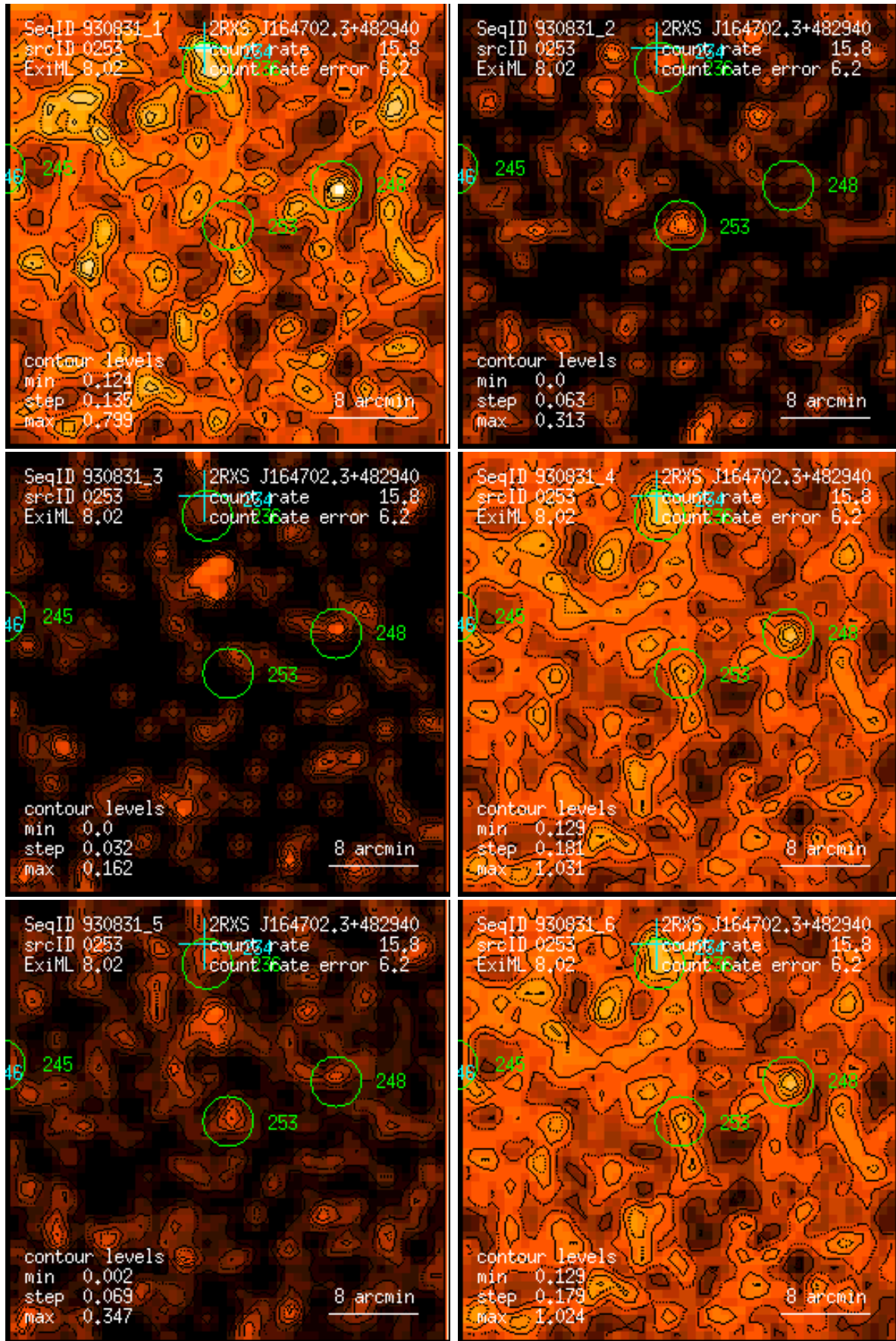
Figure 253: RASS 930831: detection 0253: band rate images, Gaussian filter: (1) PSPC channels 11 – 41, (2) 52 – 90, (3) 91 – 201, (4) 11 – 235, (5) 52 – 201, (6) 11 – 201. Broad band rates in counts/ks. Band rate contour levels in counts/ks/arcmin 2 .
