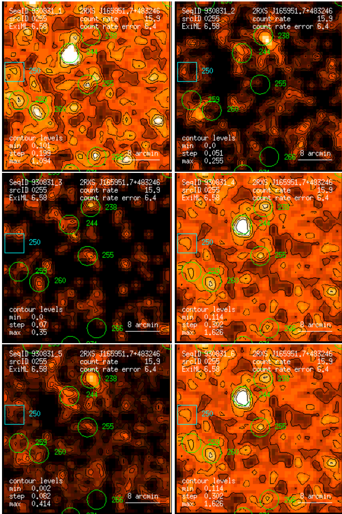
Figure 255: RASS 930831: detection 0255: band rate images, Gaussian filter: (1) PSPC channels 11 – 41, (2) 52 – 90, (3) 91 – 201, (4) 11 – 235, (5) 52 – 201, (6) 11 – 201. Broad band rates in counts/ks. Band rate contour levels in counts/ks/arcmin 2 .
