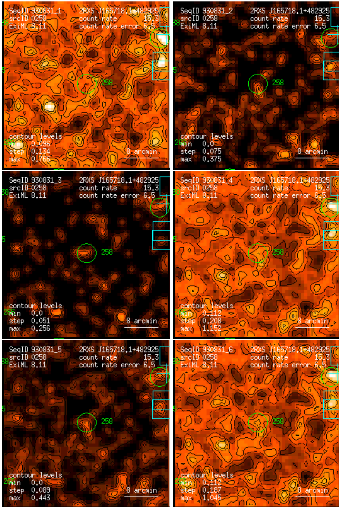
Figure 258: RASS 930831: detection 0258: band rate images, Gaussian filter: (1) PSPC channels 11 – 41, (2) 52 – 90, (3) 91 – 201, (4) 11 – 235, (5) 52 – 201, (6) 11 – 201. Broad band rates in counts/ks. Band rate contour levels in counts/ks/arcmin 2 .
