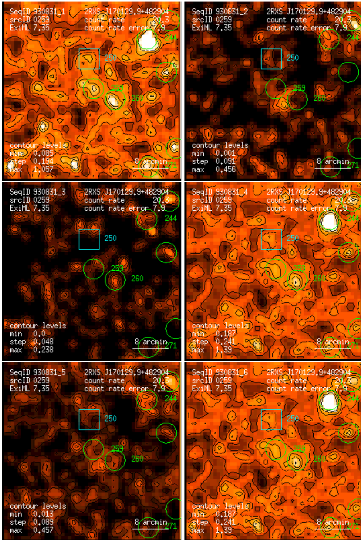
Figure 259: RASS 930831: detection 0259: band rate images, Gaussian filter: (1) PSPC channels 11 – 41, (2) 52 – 90, (3) 91 – 201, (4) 11 – 235, (5) 52 – 201, (6) 11 – 201. Broad band rates in counts/ks. Band rate contour levels in counts/ks/arcmin 2 .
