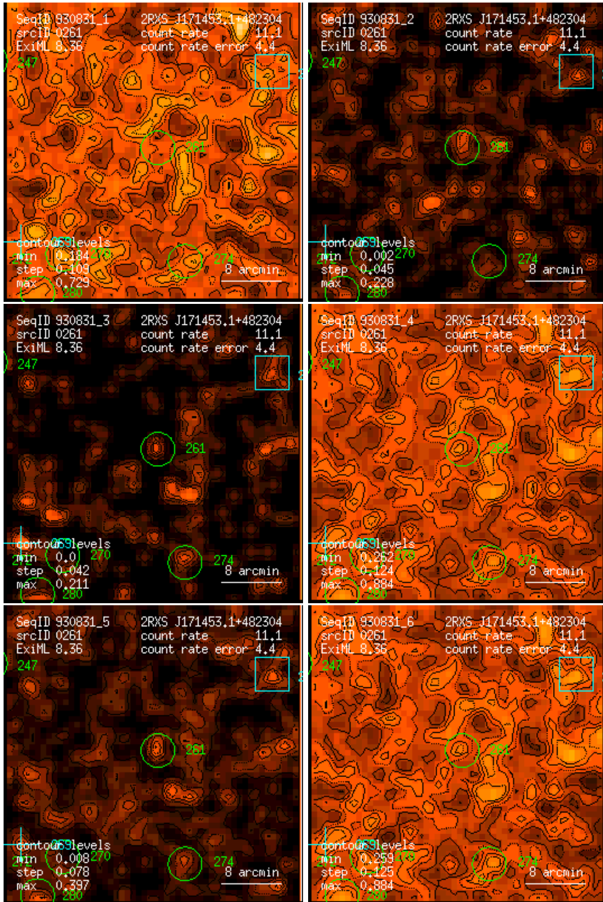
Figure 261: RASS 930831: detection 0261: band rate images, Gaussian filter: (1) PSPC channels 11 – 41, (2) 52 – 90, (3) 91 – 201, (4) 11 – 235, (5) 52 – 201, (6) 11 – 201. Broad band rates in counts/ks. Band rate contour levels in counts/ks/arcmin 2 .
