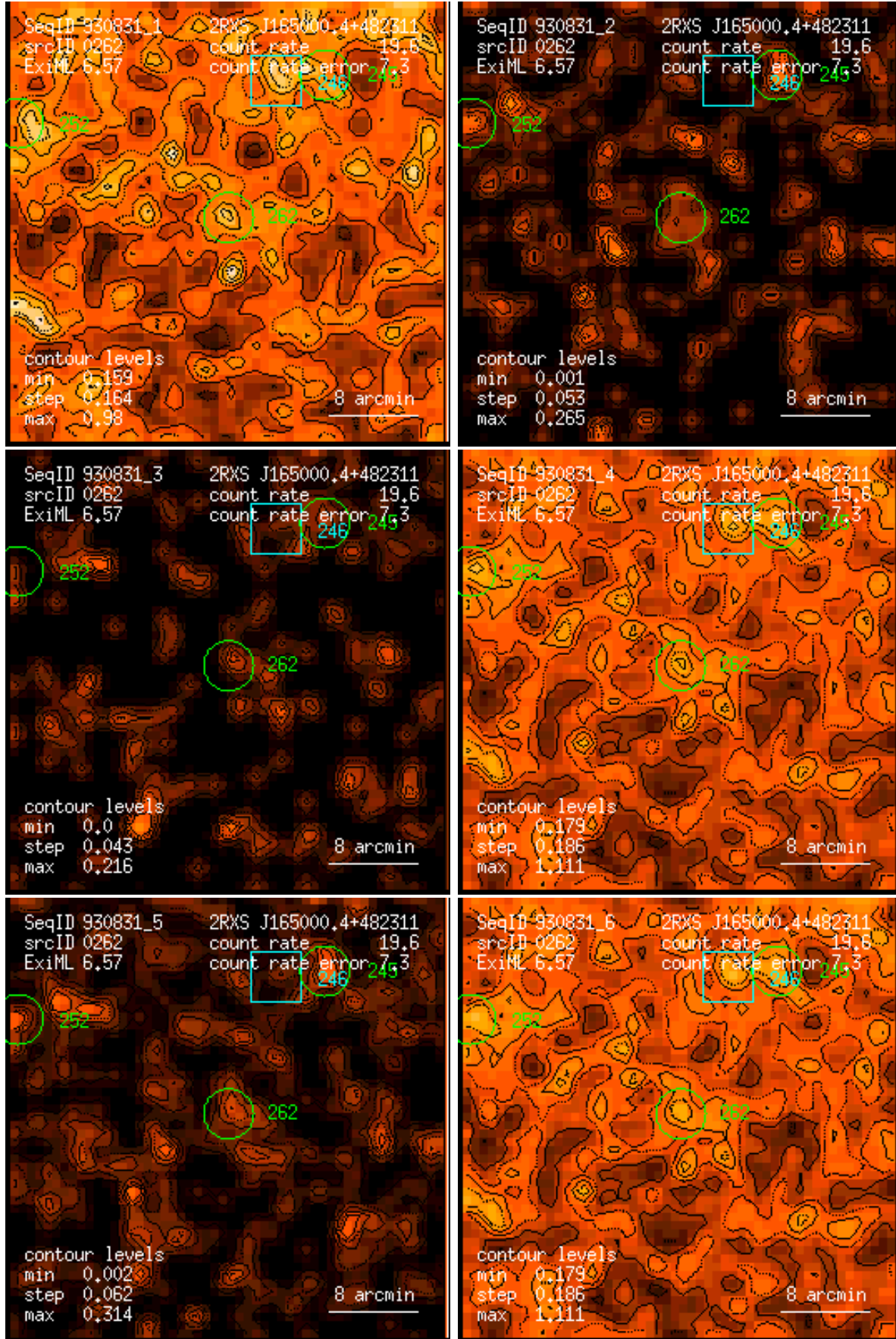
Figure 262: RASS 930831: detection 0262: band rate images, Gaussian filter: (1) PSPC channels 11 – 41, (2) 52 – 90, (3) 91 – 201, (4) 11 – 235, (5) 52 – 201, (6) 11 – 201. Broad band rates in counts/ks. Band rate contour levels in counts/ks/arcmin 2 .
