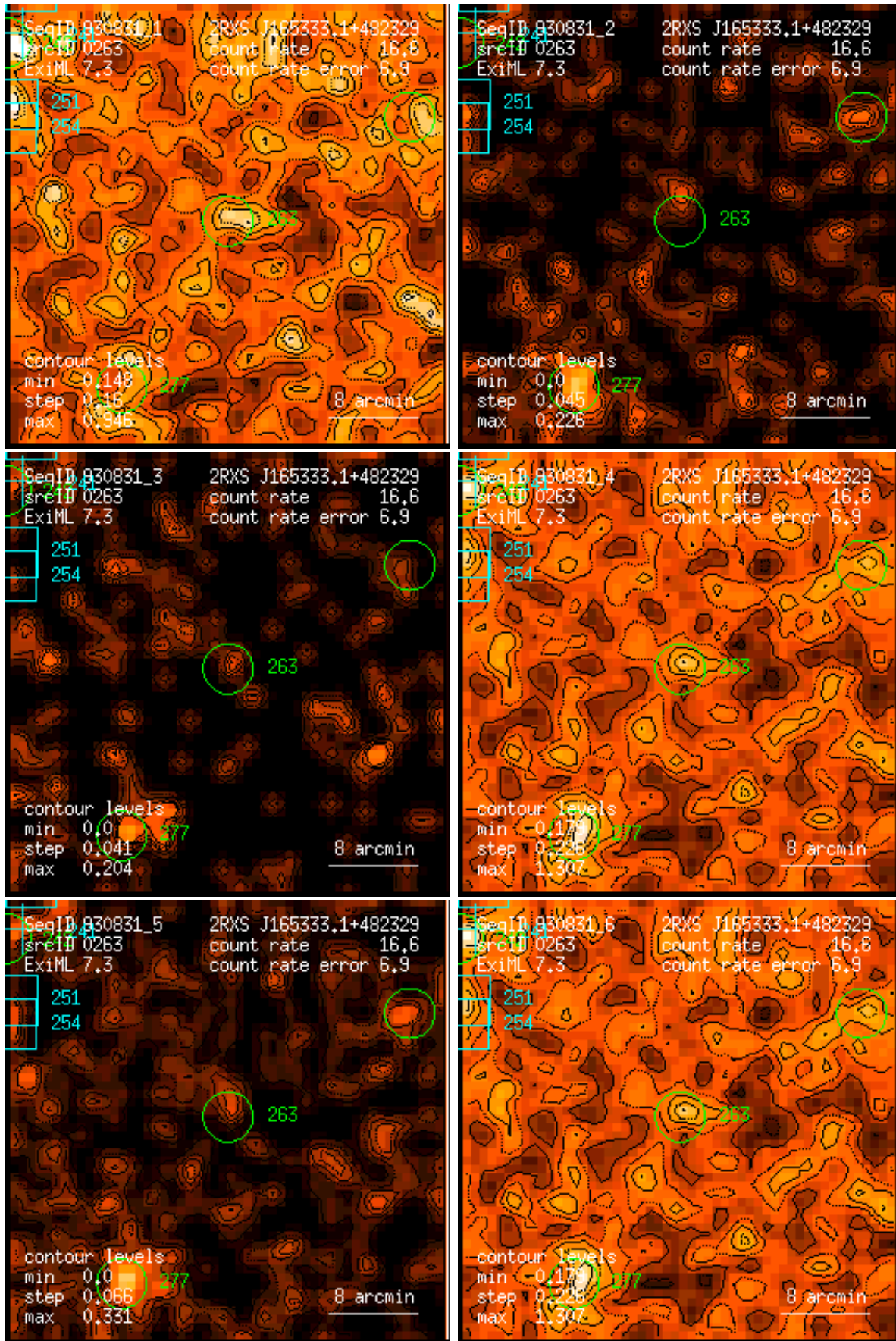
Figure 263: RASS 930831: detection 0263: band rate images, Gaussian filter: (1) PSPC channels 11 – 41, (2) 52 – 90, (3) 91 – 201, (4) 11 – 235, (5) 52 – 201, (6) 11 – 201. Broad band rates in counts/ks. Band rate contour levels in counts/ks/arcmin 2 .
