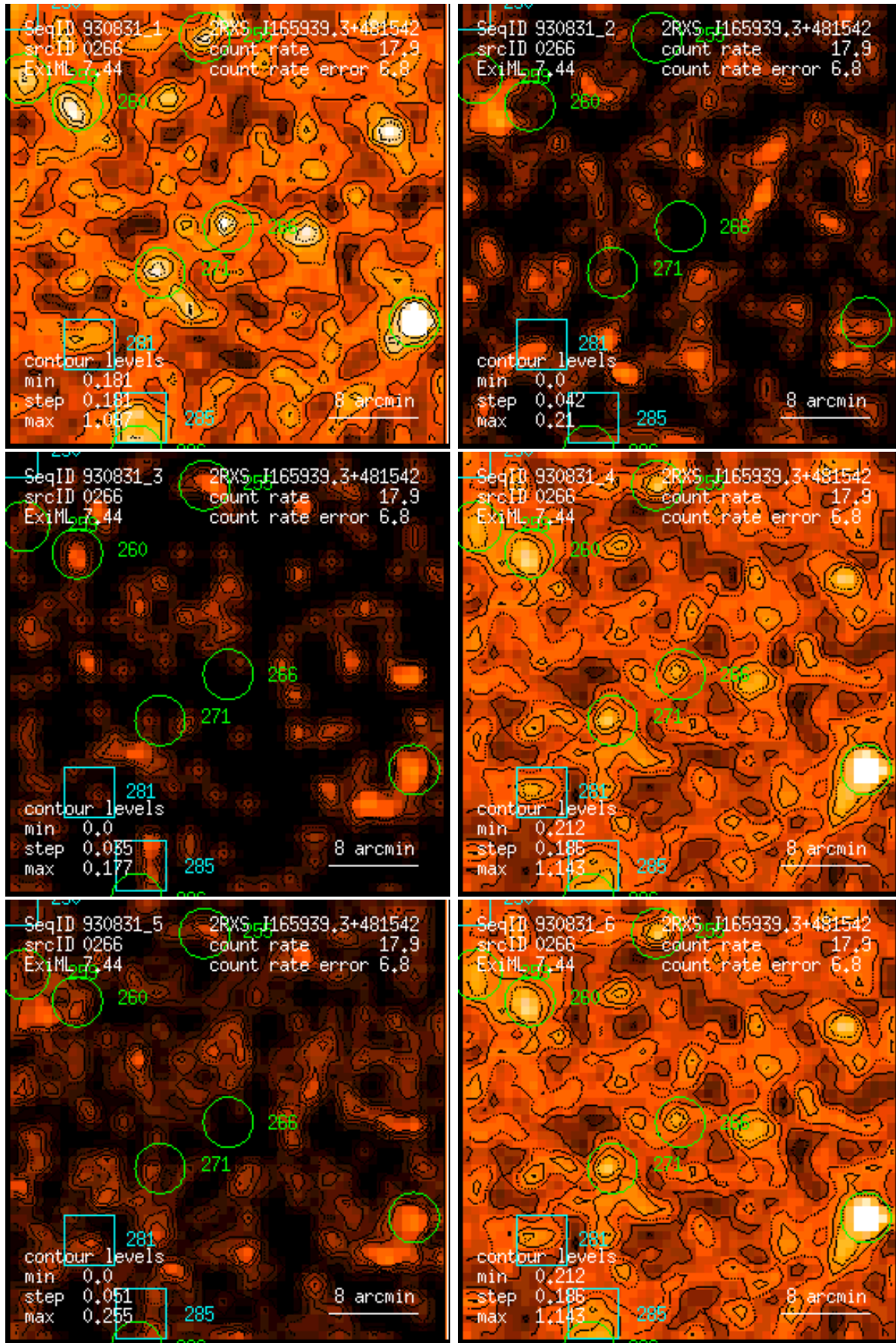
Figure 266: RASS 930831: detection 0266: band rate images, Gaussian filter: (1) PSPC channels 11 – 41, (2) 52 – 90, (3) 91 – 201, (4) 11 – 235, (5) 52 – 201, (6) 11 – 201. Broad band rates in counts/ks. Band rate contour levels in counts/ks/arcmin 2 .
