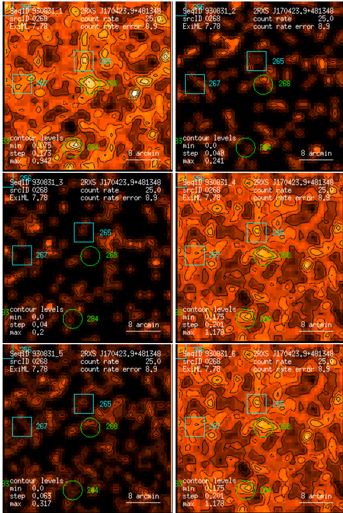
Figure 268: RASS 930831: detection 0268: band rate images, Gaussian filter: (1) PSPC channels 11 – 41, (2) 52 – 90, (3) 91 – 201, (4) 11 – 235, (5) 52 – 201, (6) 11 – 201. Broad band rates in counts/ks. Band rate contour levels in counts/ks/arcmin 2 .
