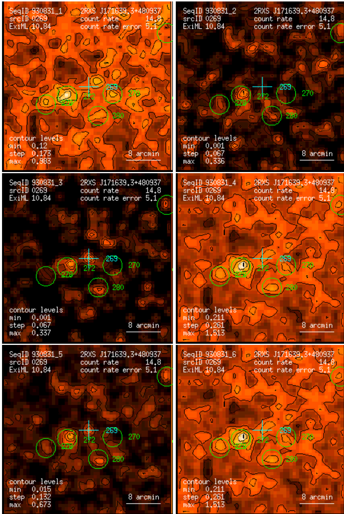
Figure 269: RASS 930831: detection 0269: band rate images, Gaussian filter: (1) PSPC channels 11 – 41, (2) 52 – 90, (3) 91 – 201, (4) 11 – 235, (5) 52 – 201, (6) 11 – 201. Broad band rates in counts/ks. Band rate contour levels in counts/ks/arcmin 2 .
