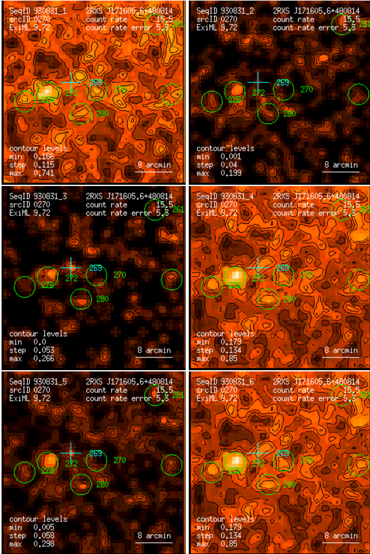
Figure 270: RASS 930831: detection 0270: band rate images, Gaussian filter: (1) PSPC channels 11 – 41, (2) 52 – 90, (3) 91 – 201, (4) 11 – 235, (5) 52 – 201, (6) 11 – 201. Broad band rates in counts/ks. Band rate contour levels in counts/ks/arcmin 2 .
