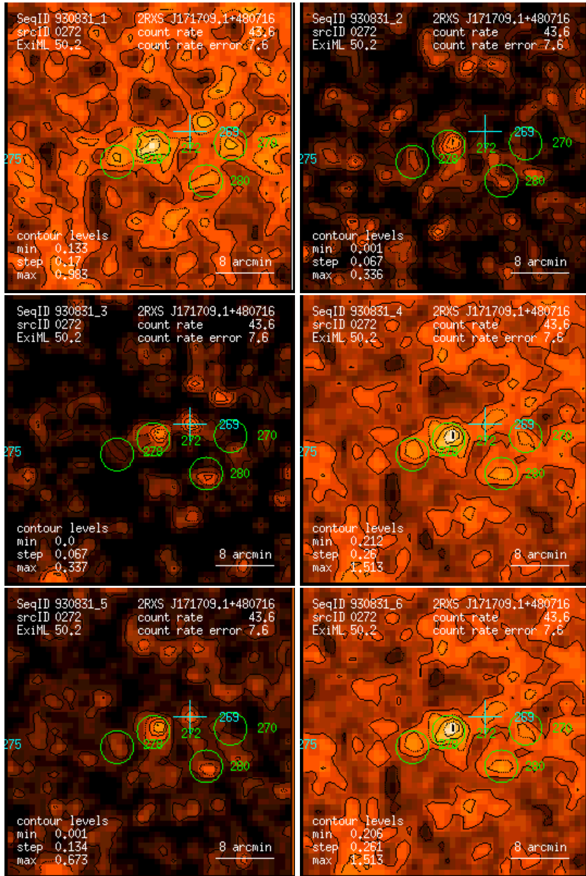
Figure 272: RASS 930831: detection 0272: band rate images, Gaussian filter: (1) PSPC channels 11 – 41, (2) 52 – 90, (3) 91 – 201, (4) 11 – 235, (5) 52 – 201, (6) 11 – 201. Broad band rates in counts/ks. Band rate contour levels in counts/ks/arcmin 2 .
