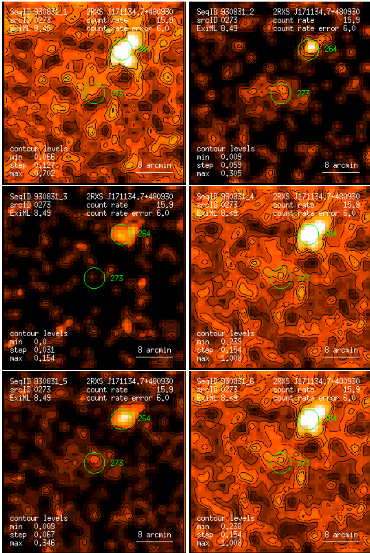
Figure 273: RASS 930831: detection 0273: band rate images, Gaussian filter: (1) PSPC channels 11 – 41, (2) 52 – 90, (3) 91 – 201, (4) 11 – 235, (5) 52 – 201, (6) 11 – 201. Broad band rates in counts/ks. Band rate contour levels in counts/ks/arcmin 2 .
