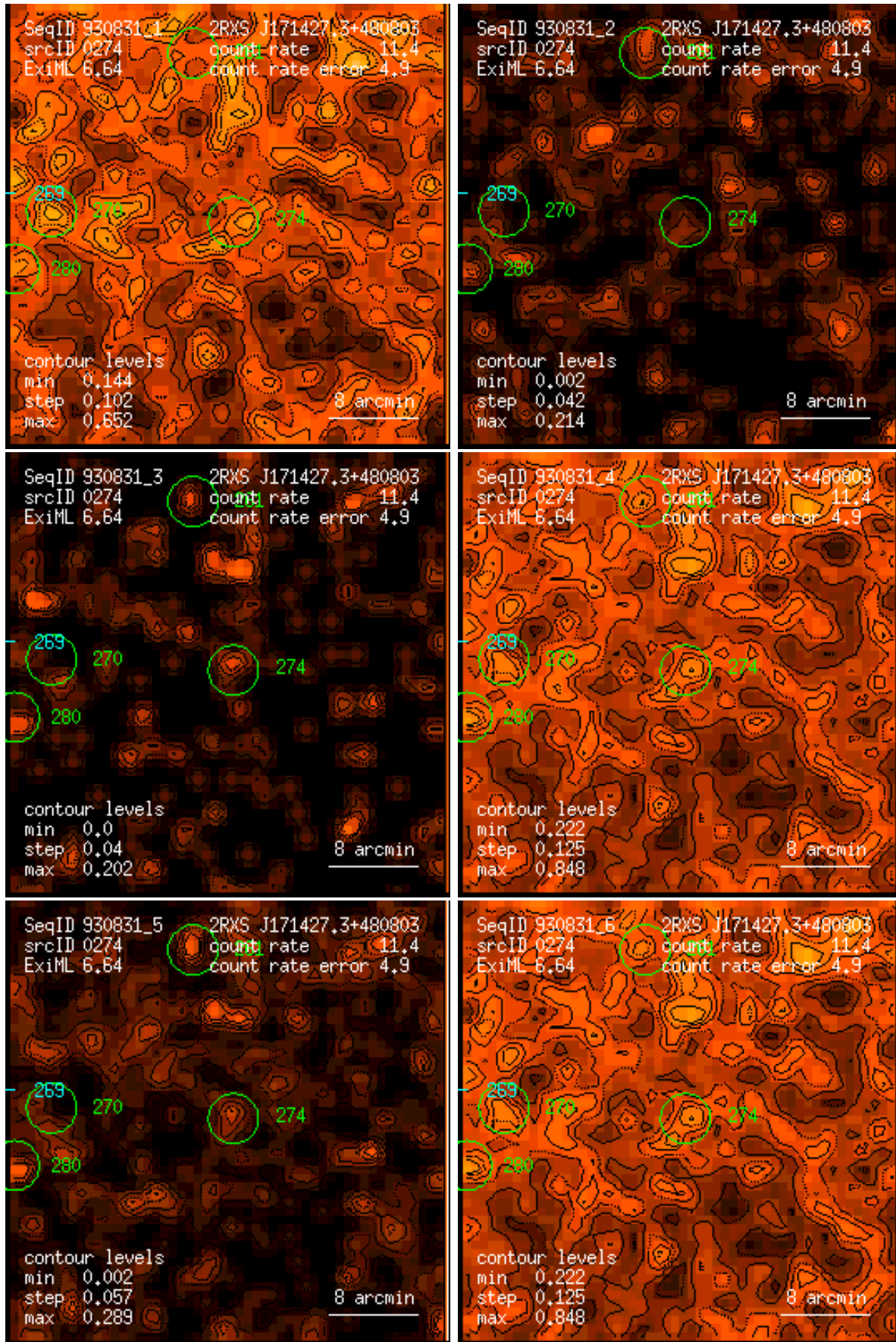
Figure 274: RASS 930831: detection 0274: band rate images, Gaussian filter: (1) PSPC channels 11 – 41, (2) 52 – 90, (3) 91 – 201, (4) 11 – 235, (5) 52 – 201, (6) 11 – 201. Broad band rates in counts/ks. Band rate contour levels in counts/ks/arcmin 2 .
