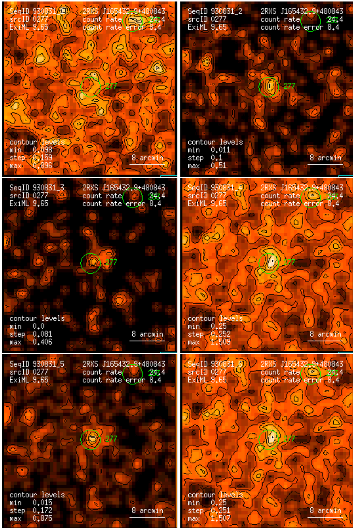
Figure 277: RASS 930831: detection 0277: band rate images, Gaussian filter: (1) PSPC channels 11 – 41, (2) 52 – 90, (3) 91 – 201, (4) 11 – 235, (5) 52 – 201, (6) 11 – 201. Broad band rates in counts/ks. Band rate contour levels in counts/ks/arcmin 2 .
