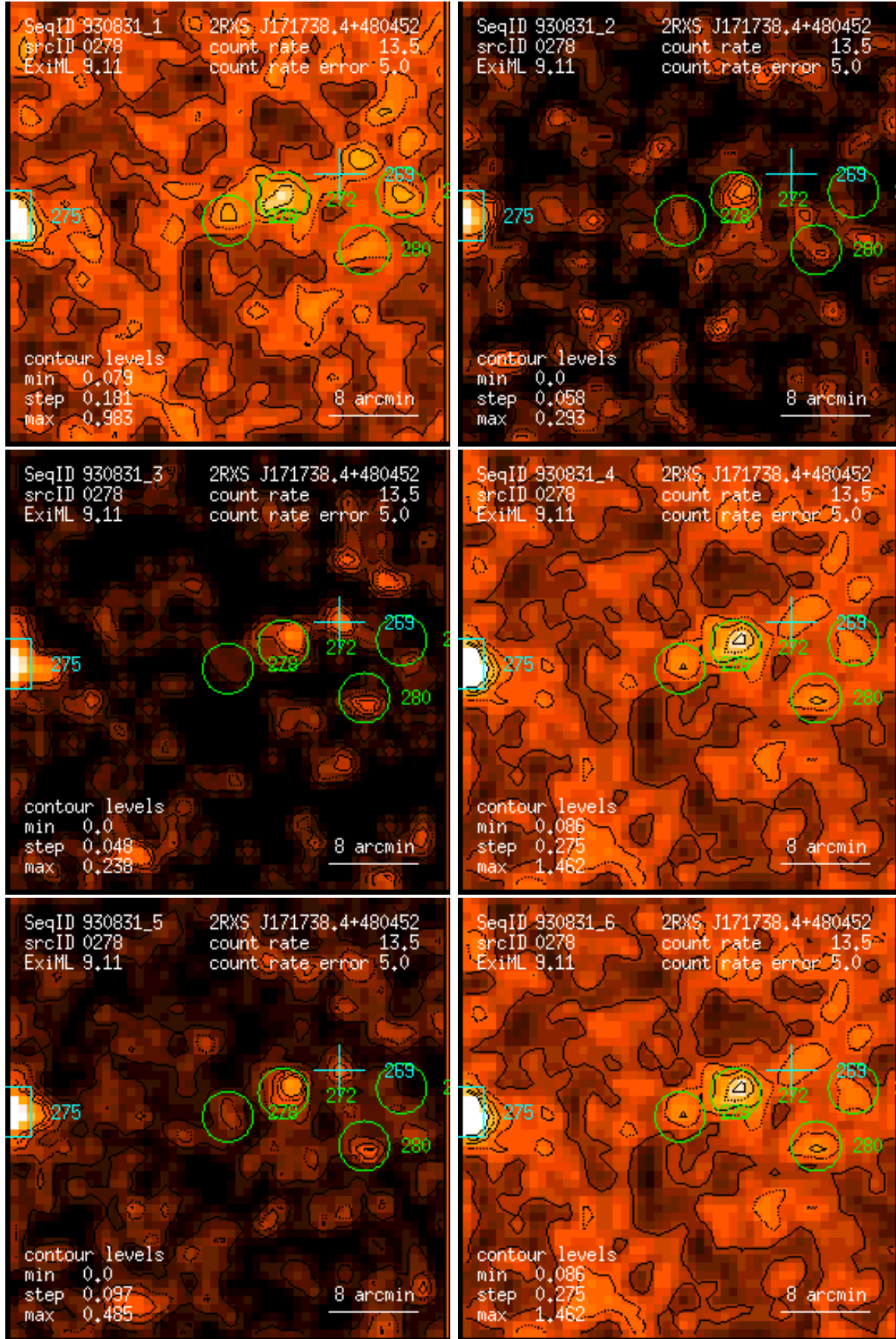
Figure 278: RASS 930831: detection 0278: band rate images, Gaussian filter: (1) PSPC channels 11 – 41, (2) 52 – 90, (3) 91 – 201, (4) 11 – 235, (5) 52 – 201, (6) 11 – 201. Broad band rates in counts/ks. Band rate contour levels in counts/ks/arcmin 2 .
