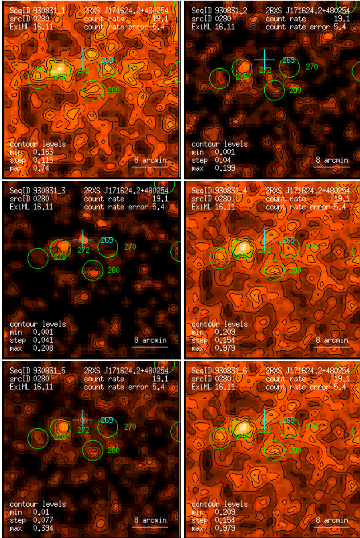
Figure 280: RASS 930831: detection 0280: band rate images, Gaussian filter: (1) PSPC channels 11 – 41, (2) 52 – 90, (3) 91 – 201, (4) 11 – 235, (5) 52 – 201, (6) 11 – 201. Broad band rates in counts/ks. Band rate contour levels in counts/ks/arcmin 2 .
