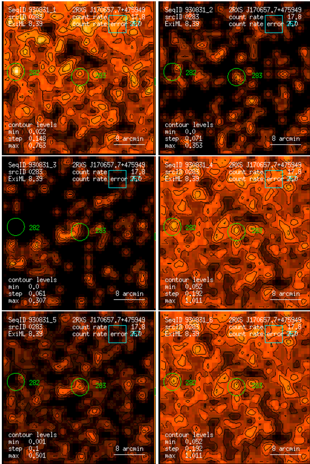
Figure 283: RASS 930831: detection 0283: band rate images, Gaussian filter: (1) PSPC channels 11 – 41, (2) 52 – 90, (3) 91 – 201, (4) 11 – 235, (5) 52 – 201, (6) 11 – 201. Broad band rates in counts/ks. Band rate contour levels in counts/ks/arcmin 2 .
