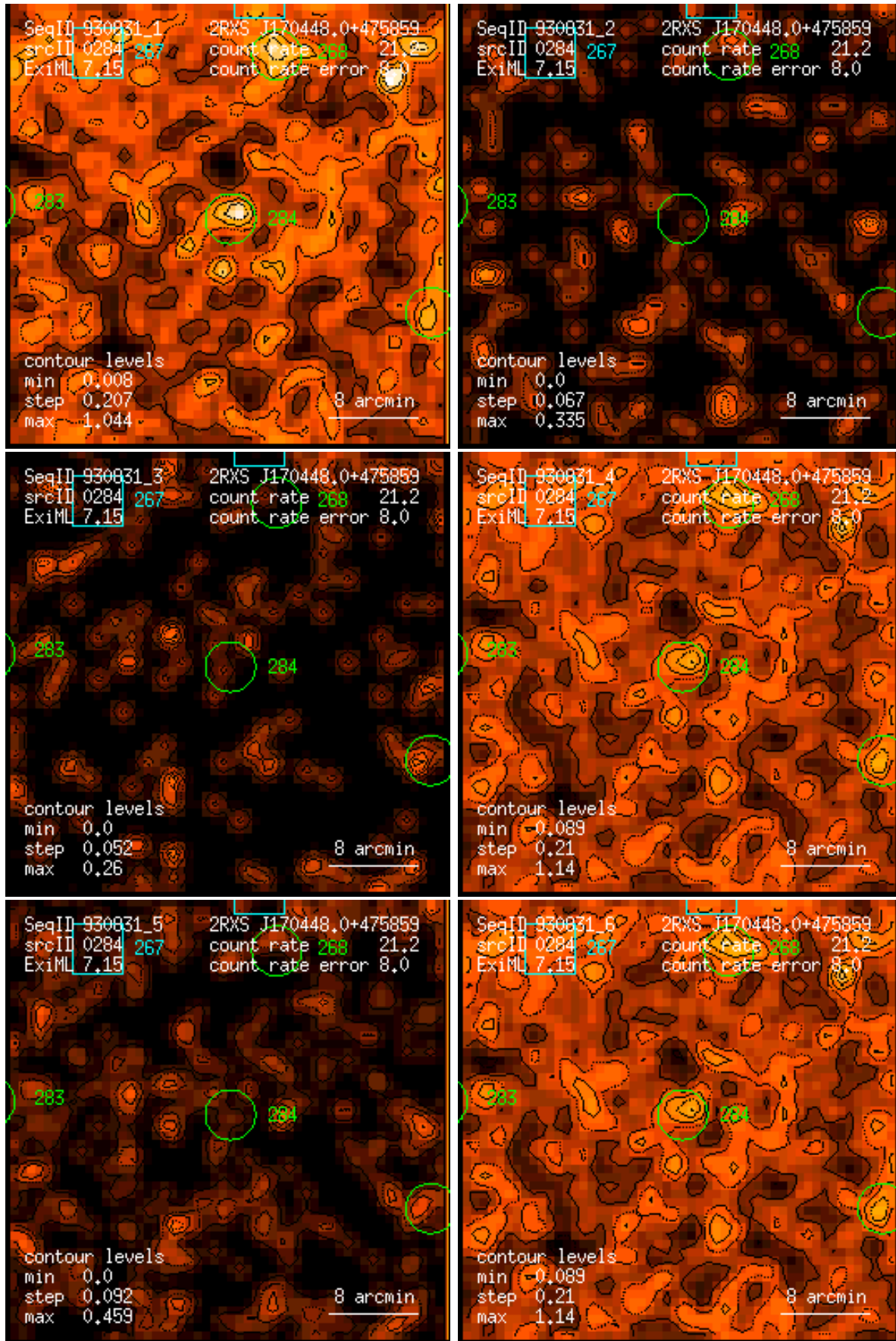
Figure 284: RASS 930831: detection 0284: band rate images, Gaussian filter: (1) PSPC channels 11 – 41, (2) 52 – 90, (3) 91 – 201, (4) 11 – 235, (5) 52 – 201, (6) 11 – 201. Broad band rates in counts/ks. Band rate contour levels in counts/ks/arcmin 2 .
