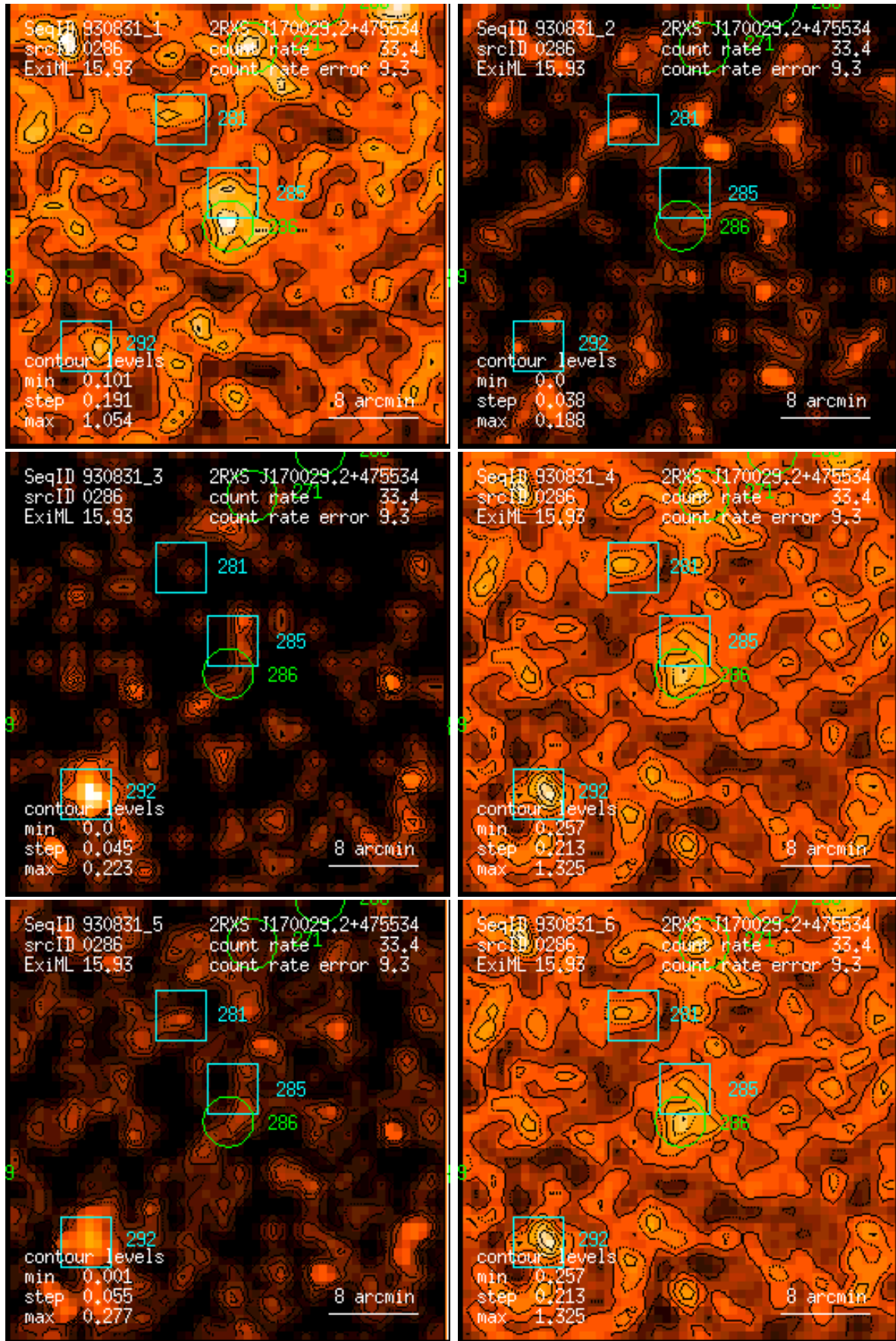
Figure 286: RASS 930831: detection 0286: band rate images, Gaussian filter: (1) PSPC channels 11 – 41, (2) 52 – 90, (3) 91 – 201, (4) 11 – 235, (5) 52 – 201, (6) 11 – 201. Broad band rates in counts/ks. Band rate contour levels in counts/ks/arcmin 2 .
