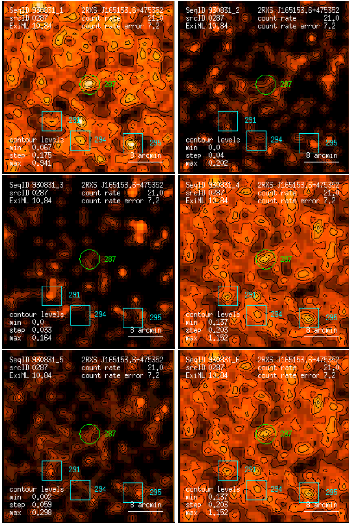
Figure 287: RASS 930831: detection 0287: band rate images, Gaussian filter: (1) PSPC channels 11 – 41, (2) 52 – 90, (3) 91 – 201, (4) 11 – 235, (5) 52 – 201, (6) 11 – 201. Broad band rates in counts/ks. Band rate contour levels in counts/ks/arcmin 2 .
