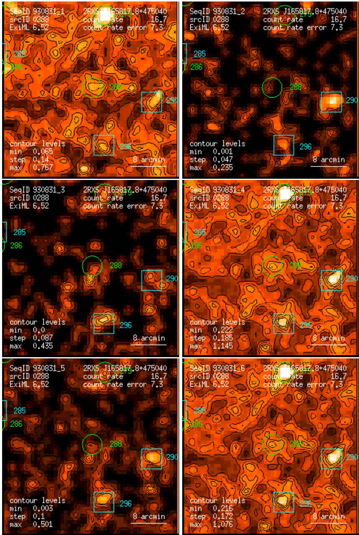
Figure 288: RASS 930831: detection 0288: band rate images, Gaussian filter: (1) PSPC channels 11 – 41, (2) 52 – 90, (3) 91 – 201, (4) 11 – 235, (5) 52 – 201, (6) 11 – 201. Broad band rates in counts/ks. Band rate contour levels in counts/ks/arcmin 2 .
