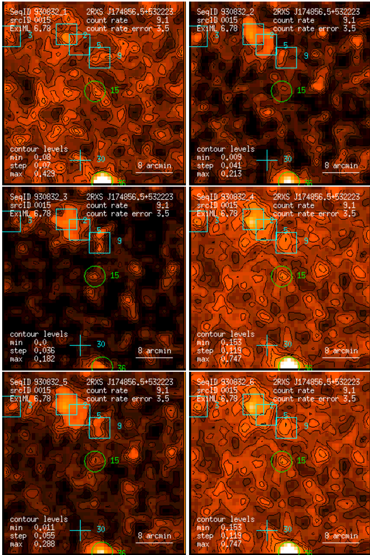
Figure 15: RASS 930832: detection 0015: band rate images, Gaussian filter: (1) PSPC channels 11 – 41, (2) 52 – 90, (3) 91 – 201, (4) 11 – 235, (5) 52 – 201, (6) 11 – 201. Broad band rates in counts/ks. Band rate contour levels in counts/ks/arcmin 2 .
