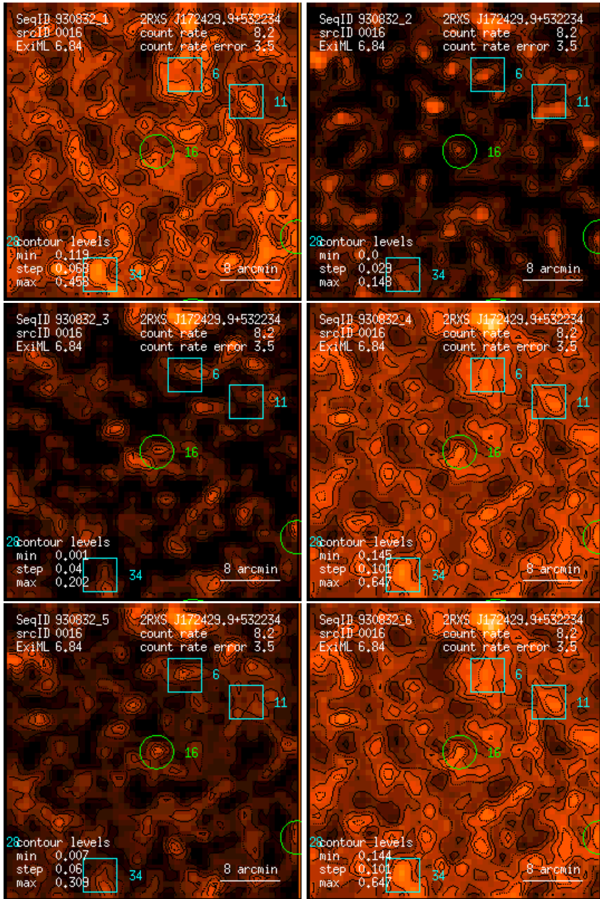
Figure 16: RASS 930832: detection 0016: band rate images, Gaussian filter: (1) PSPC channels 11 – 41, (2) 52 – 90, (3) 91 – 201, (4) 11 – 235, (5) 52 – 201, (6) 11 – 201. Broad band rates in counts/ks. Band rate contour levels in counts/ks/arcmin 2 .
