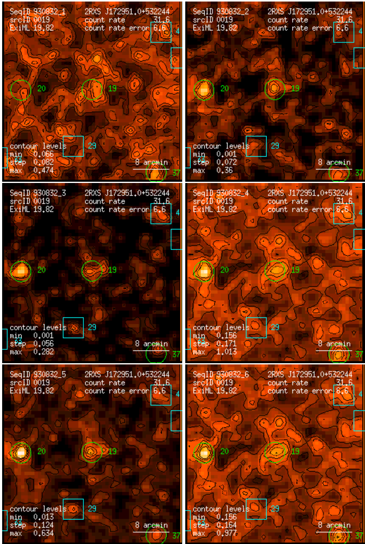
Figure 19: RASS 930832: detection 0019: band rate images, Gaussian filter: (1) PSPC channels 11 – 41, (2) 52 – 90, (3) 91 – 201, (4) 11 – 235, (5) 52 – 201, (6) 11 – 201. Broad band rates in counts/ks. Band rate contour levels in counts/ks/arcmin 2 .
