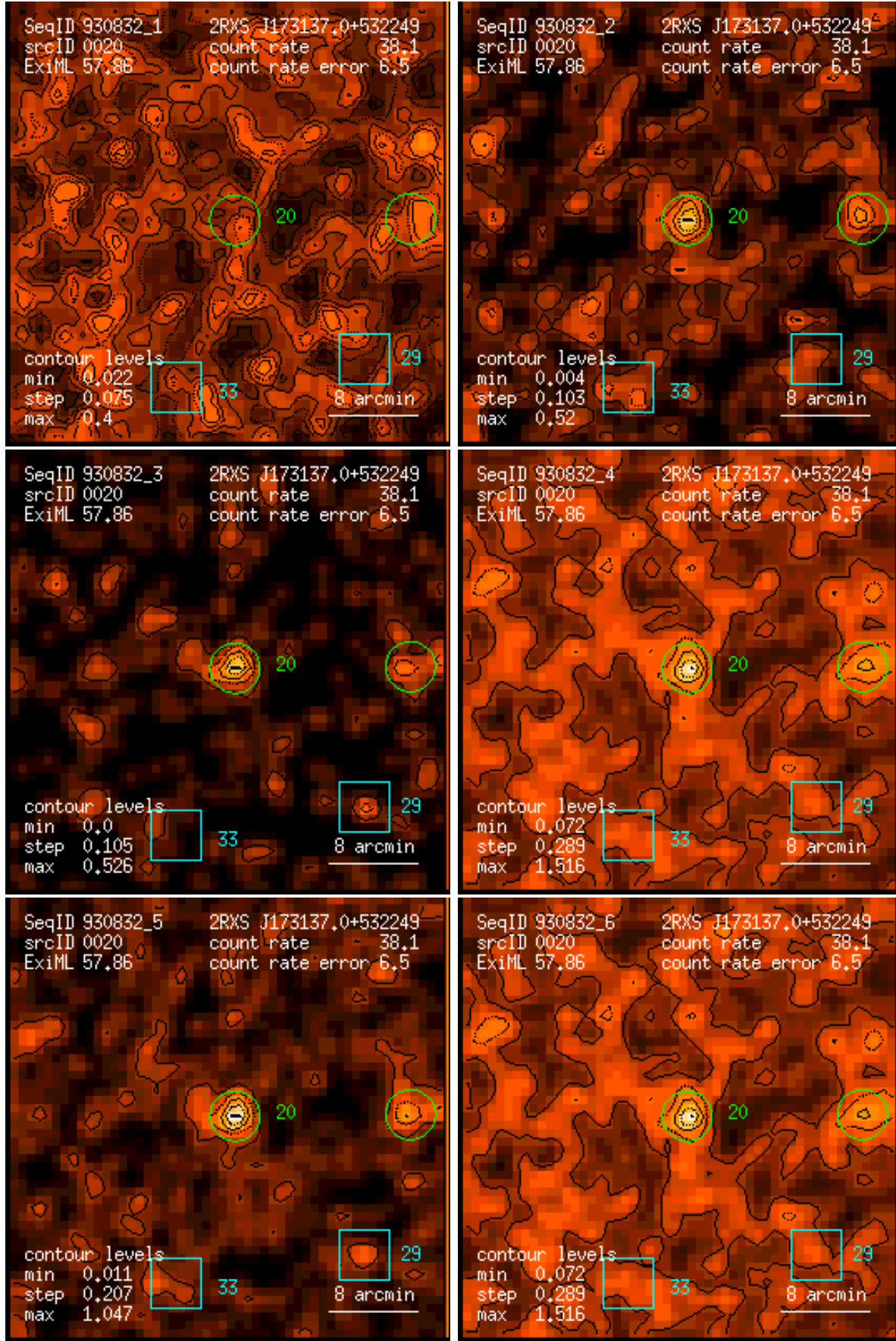
Figure 20: RASS 930832: detection 0020: band rate images, Gaussian filter: (1) PSPC channels 11 – 41, (2) 52 – 90, (3) 91 – 201, (4) 11 – 235, (5) 52 – 201, (6) 11 – 201. Broad band rates in counts/ks. Band rate contour levels in counts/ks/arcmin 2 .
