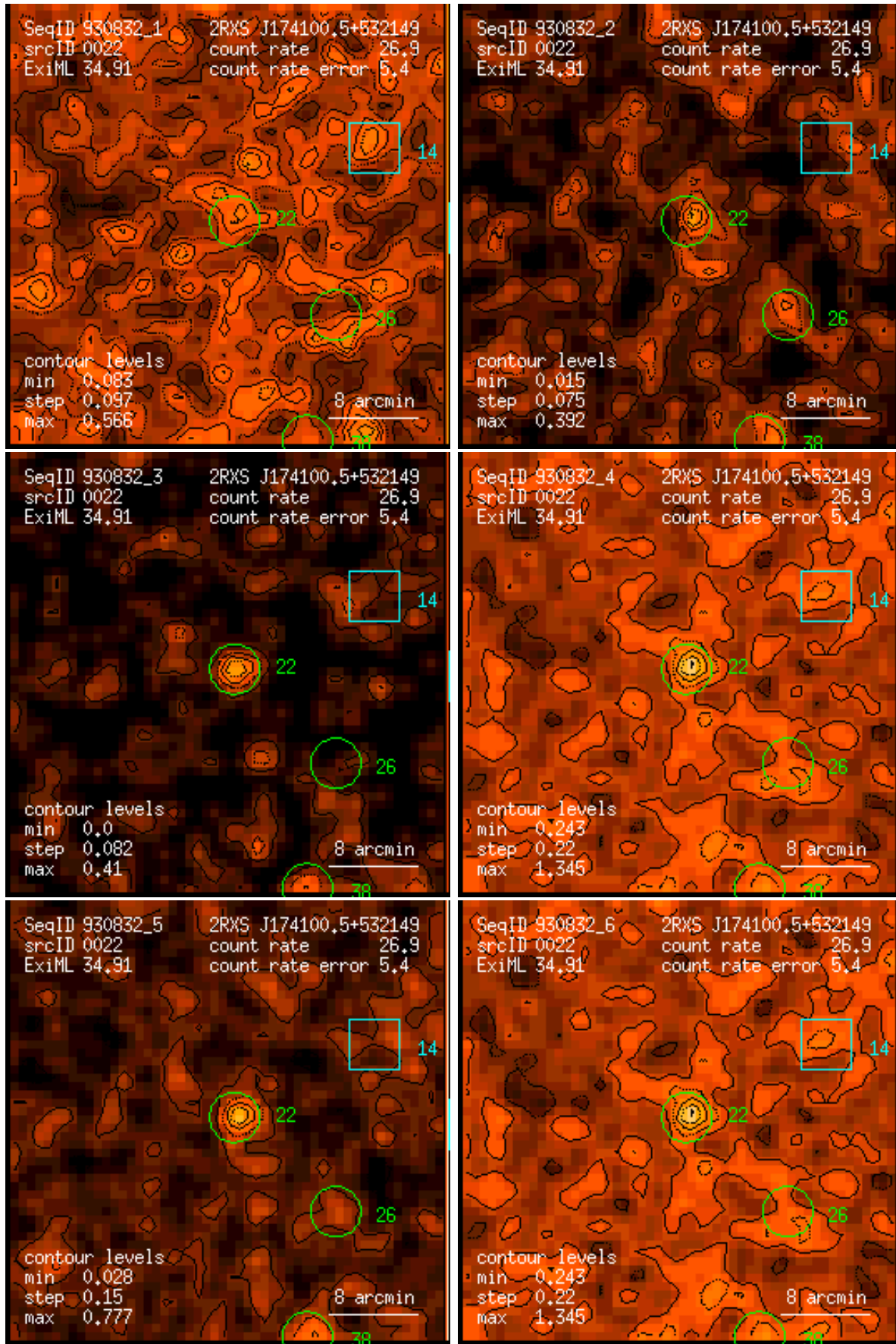
Figure 22: RASS 930832: detection 0022: band rate images, Gaussian filter: (1) PSPC channels 11 – 41, (2) 52 – 90, (3) 91 – 201, (4) 11 – 235, (5) 52 – 201, (6) 11 – 201. Broad band rates in counts/ks. Band rate contour levels in counts/ks/arcmin 2 .
