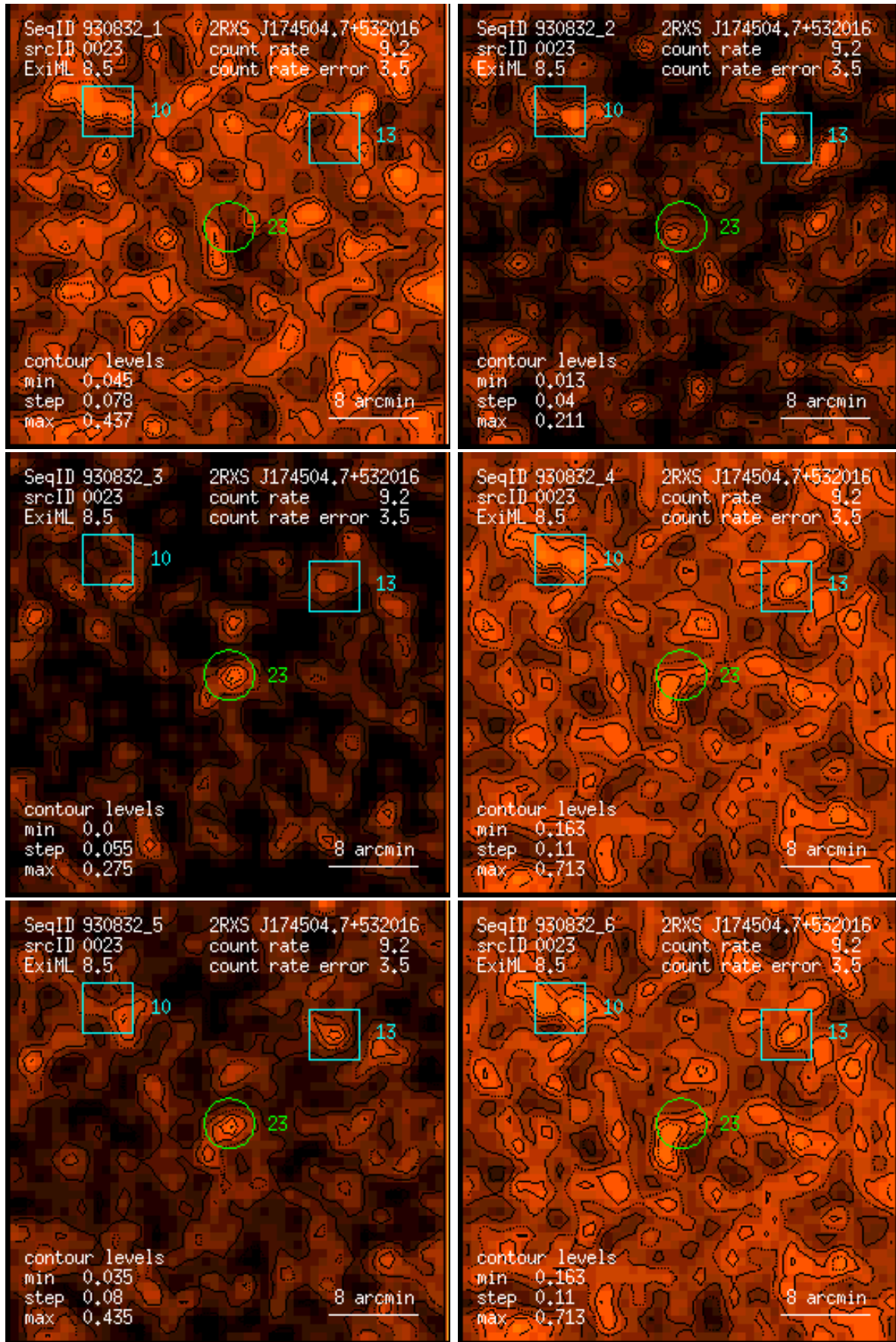
Figure 23: RASS 930832: detection 0023: band rate images, Gaussian filter: (1) PSPC channels 11 – 41, (2) 52 – 90, (3) 91 – 201, (4) 11 – 235, (5) 52 – 201, (6) 11 – 201. Broad band rates in counts/ks. Band rate contour levels in counts/ks/arcmin 2 .
