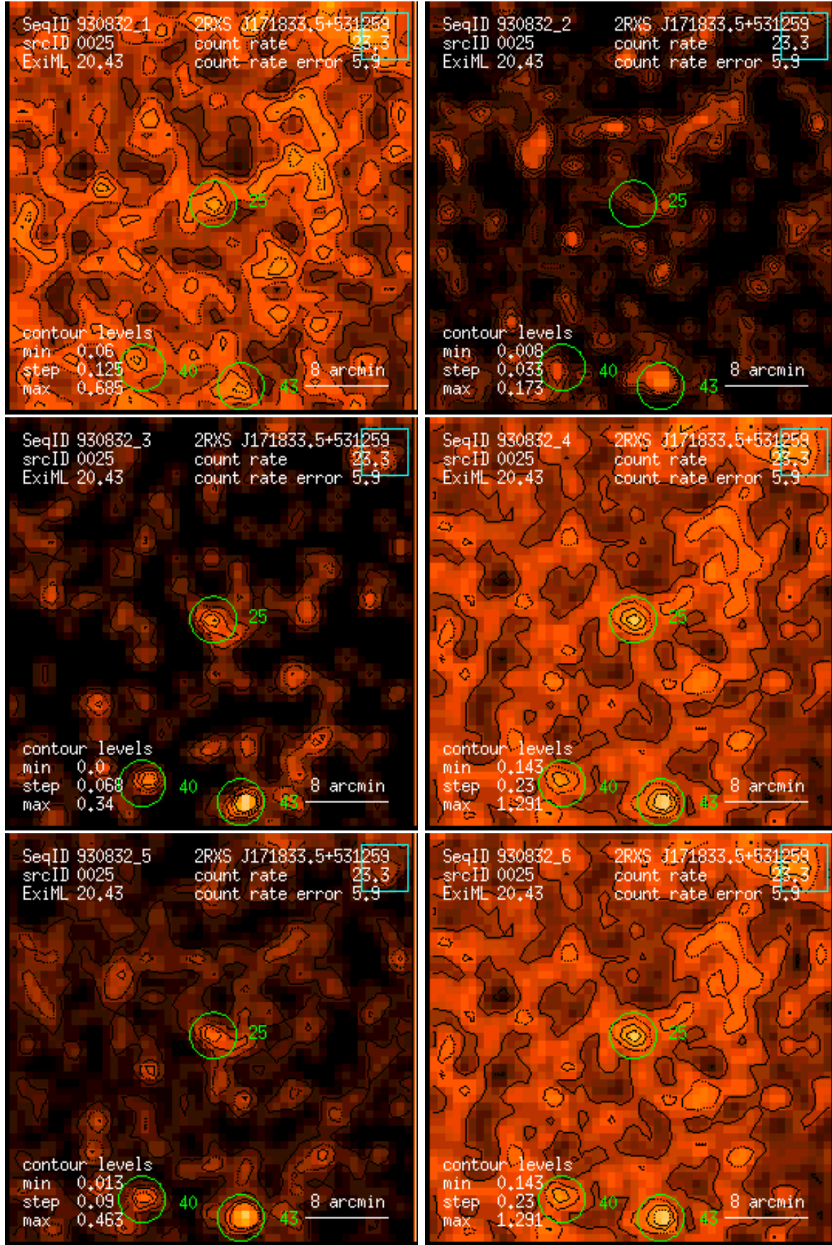
Figure 25: RASS 930832: detection 0025: band rate images, Gaussian filter: (1) PSPC channels 11 – 41, (2) 52 – 90, (3) 91 – 201, (4) 11 – 235, (5) 52 – 201, (6) 11 – 201. Broad band rates in counts/ks. Band rate contour levels in counts/ks/arcmin 2 .
