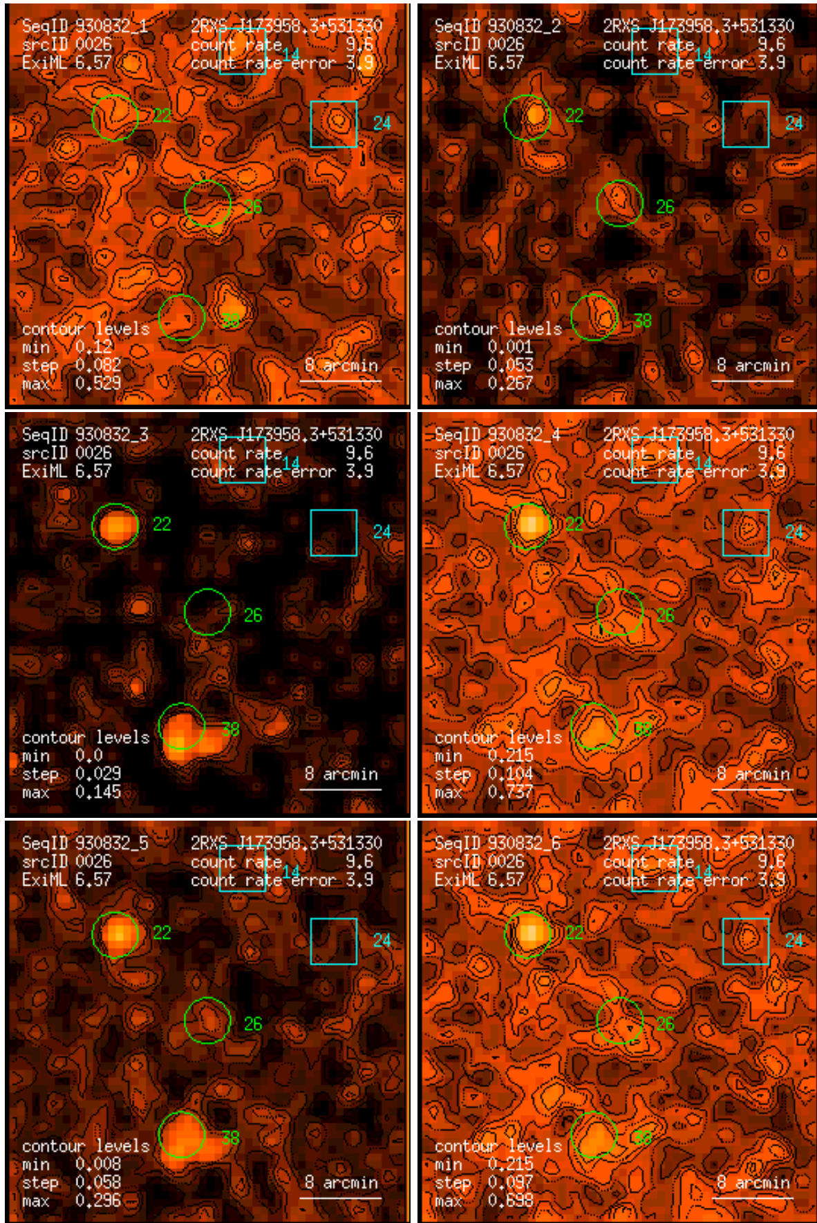
Figure 26: RASS 930832: detection 0026: band rate images, Gaussian filter: (1) PSPC channels 11 – 41, (2) 52 – 90, (3) 91 – 201, (4) 11 – 235, (5) 52 – 201, (6) 11 – 201. Broad band rates in counts/ks. Band rate contour levels in counts/ks/arcmin 2 .
