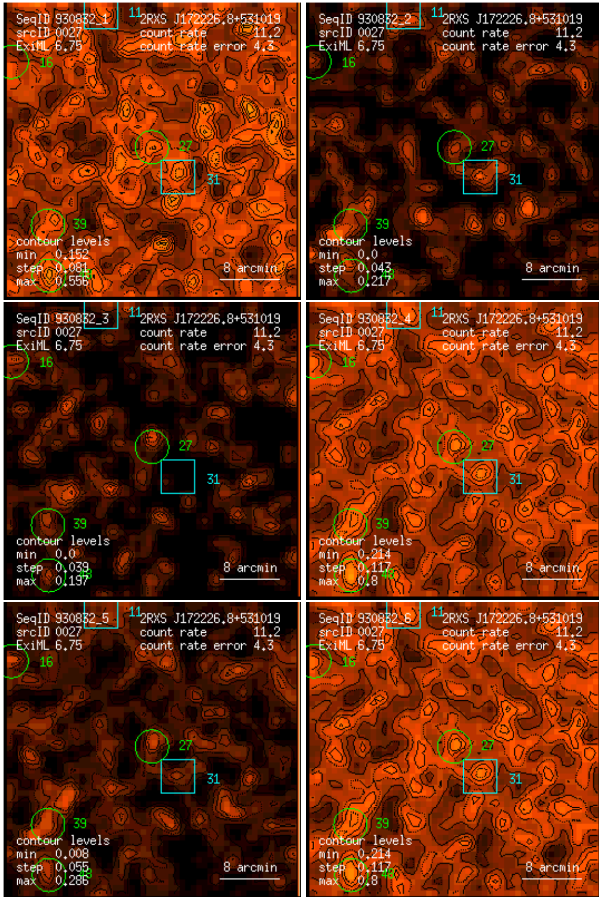
Figure 27: RASS 930832: detection 0027: band rate images, Gaussian filter: (1) PSPC channels 11 – 41, (2) 52 – 90, (3) 91 – 201, (4) 11 – 235, (5) 52 – 201, (6) 11 – 201. Broad band rates in counts/ks. Band rate contour levels in counts/ks/arcmin 2 .
