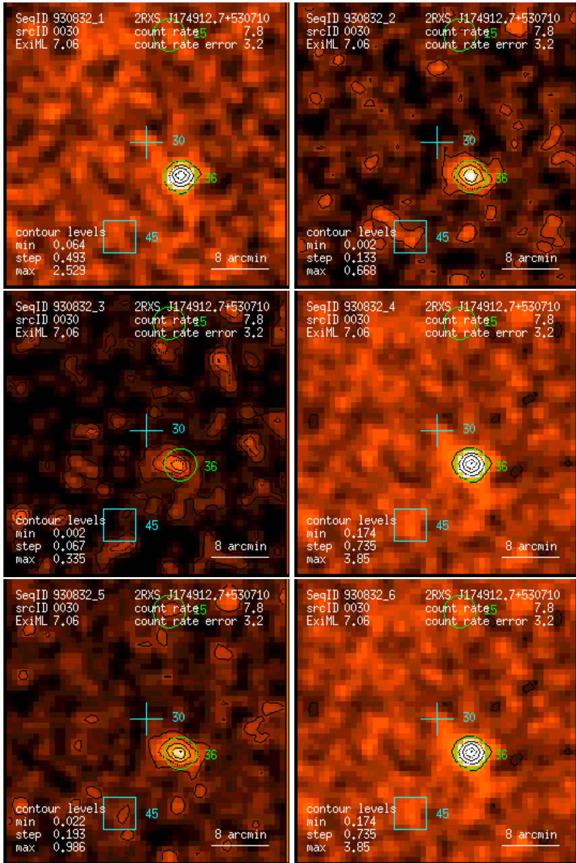
Figure 30: RASS 930832: detection 0030: band rate images, Gaussian filter: (1) PSPC channels 11 – 41, (2) 52 – 90, (3) 91 – 201, (4) 11 – 235, (5) 52 – 201, (6) 11 – 201. Broad band rates in counts/ks. Band rate contour levels in counts/ks/arcmin 2 .
