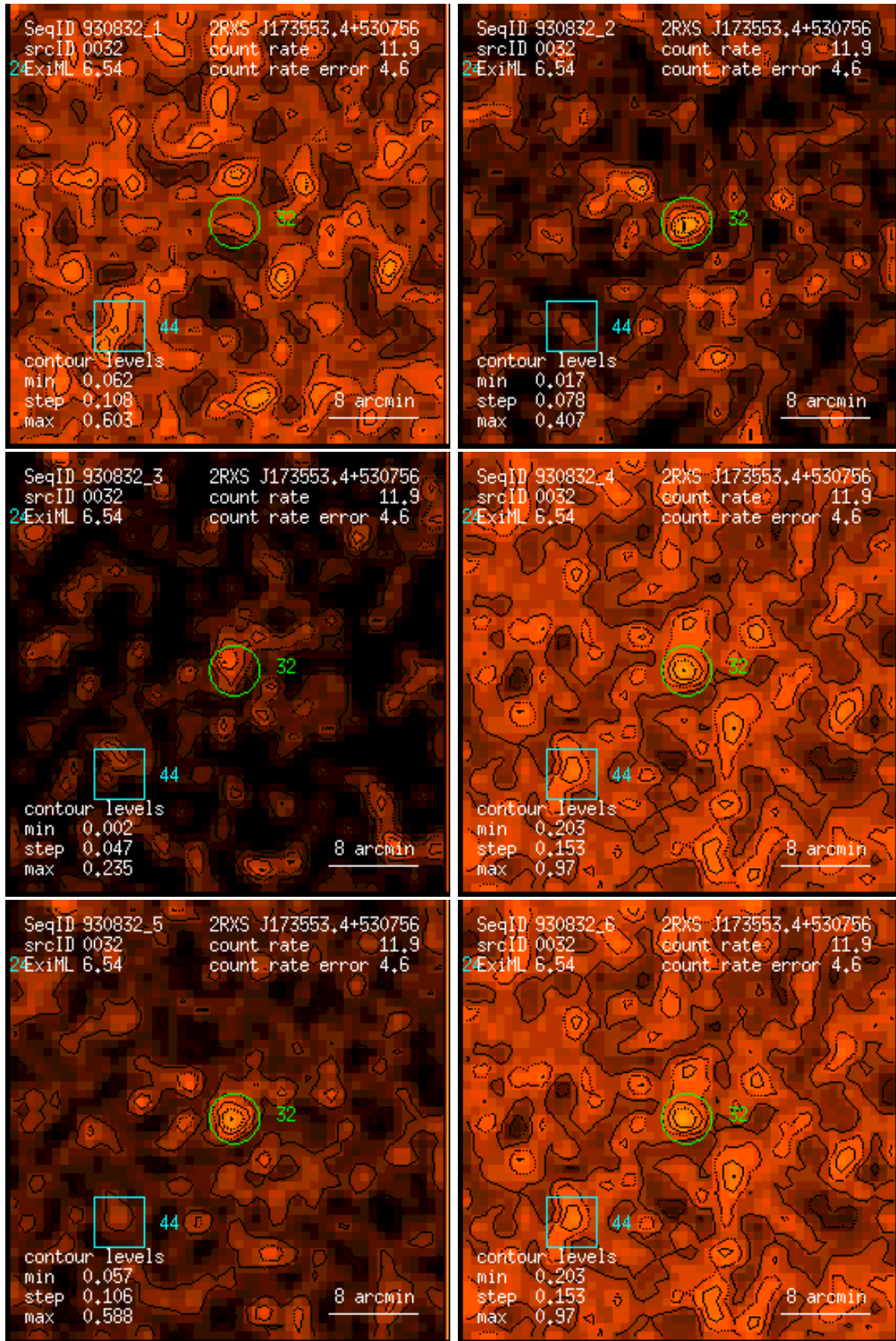
Figure 32: RASS 930832: detection 0032: band rate images, Gaussian filter: (1) PSPC channels 11 – 41, (2) 52 – 90, (3) 91 – 201, (4) 11 – 235, (5) 52 – 201, (6) 11 – 201. Broad band rates in counts/ks. Band rate contour levels in counts/ks/arcmin 2 .
