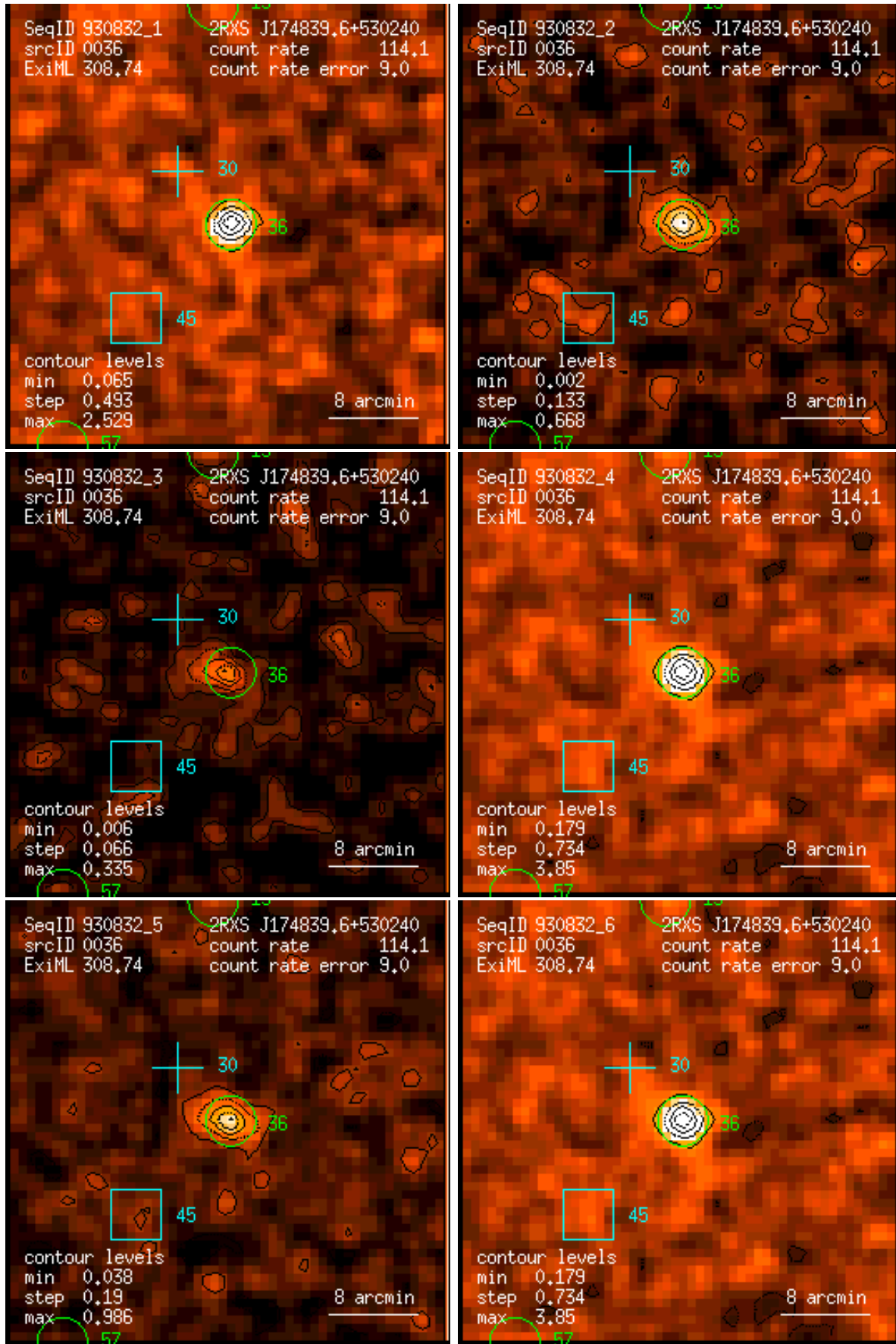
Figure 36: RASS 930832: detection 0036: band rate images, Gaussian filter: (1) PSPC channels 11 – 41, (2) 52 – 90, (3) 91 – 201, (4) 11 – 235, (5) 52 – 201, (6) 11 – 201. Broad band rates in counts/ks. Band rate contour levels in counts/ks/arcmin 2 .
