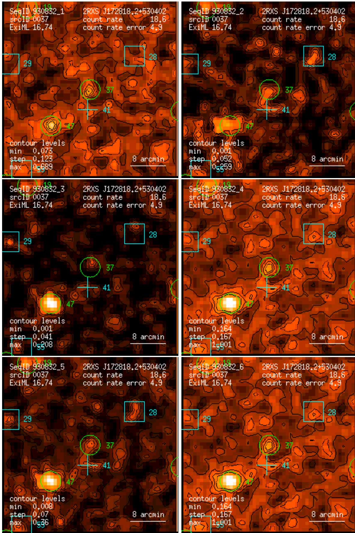
Figure 37: RASS 930832: detection 0037: band rate images, Gaussian filter: (1) PSPC channels 11 – 41, (2) 52 – 90, (3) 91 – 201, (4) 11 – 235, (5) 52 – 201, (6) 11 – 201. Broad band rates in counts/ks. Band rate contour levels in counts/ks/arcmin 2 .
