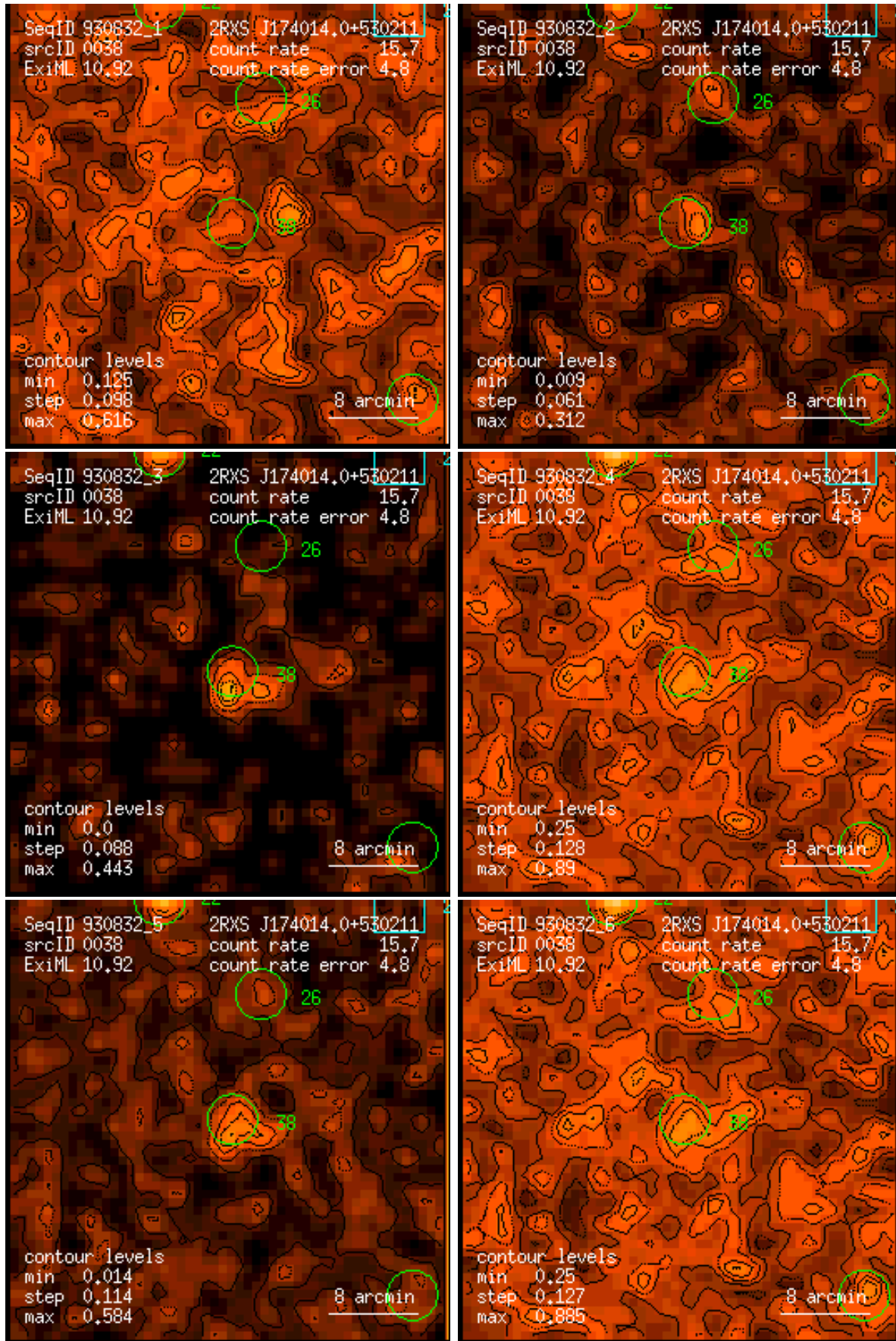
Figure 38: RASS 930832: detection 0038: band rate images, Gaussian filter: (1) PSPC channels 11 – 41, (2) 52 – 90, (3) 91 – 201, (4) 11 – 235, (5) 52 – 201, (6) 11 – 201. Broad band rates in counts/ks. Band rate contour levels in counts/ks/arcmin 2 .
