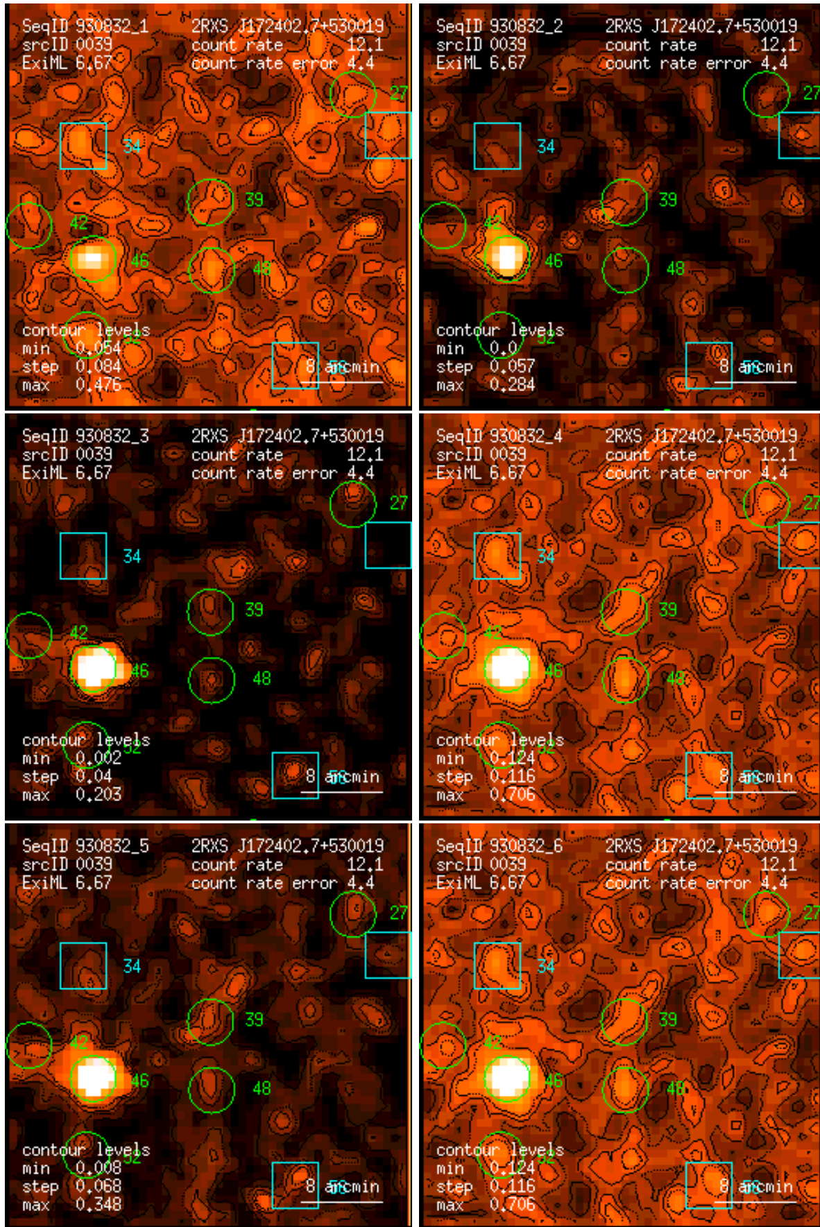
Figure 39: RASS 930832: detection 0039: band rate images, Gaussian filter: (1) PSPC channels 11 – 41, (2) 52 – 90, (3) 91 – 201, (4) 11 – 235, (5) 52 – 201, (6) 11 – 201. Broad band rates in counts/ks. Band rate contour levels in counts/ks/arcmin 2 .
