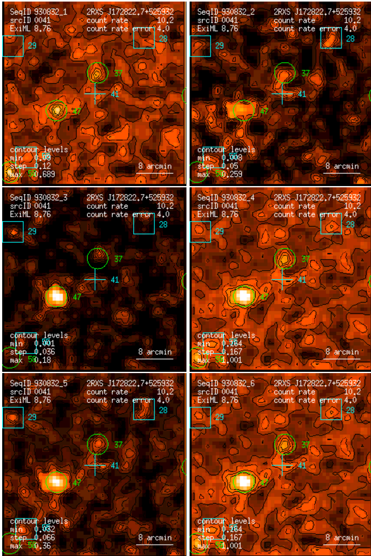
Figure 41: RASS 930832: detection 0041: band rate images, Gaussian filter: (1) PSPC channels 11 – 41, (2) 52 – 90, (3) 91 – 201, (4) 11 – 235, (5) 52 – 201, (6) 11 – 201. Broad band rates in counts/ks. Band rate contour levels in counts/ks/arcmin 2 .
